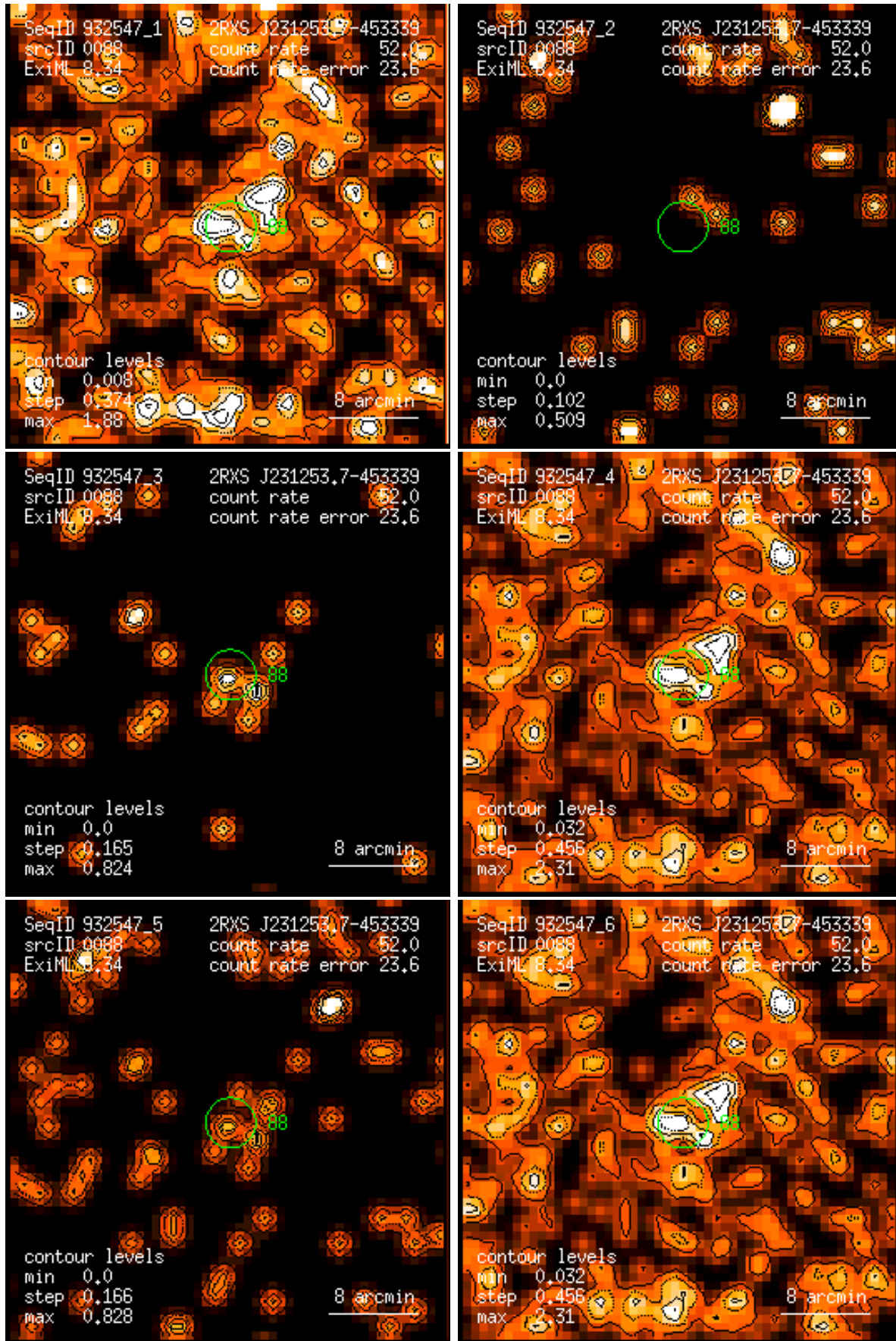
Figure 88: RASS 932547: detection 0088: band rate images, Gaussian filter: (1) PSPC channels 11 – 41, (2) 52 – 90, (3) 91 – 201, (4) 11 – 235, (5) 52 – 201, (6) 11 – 201. Broad band rates in counts/ks. Band rate contour levels in counts/ks/arcmin 2 .
