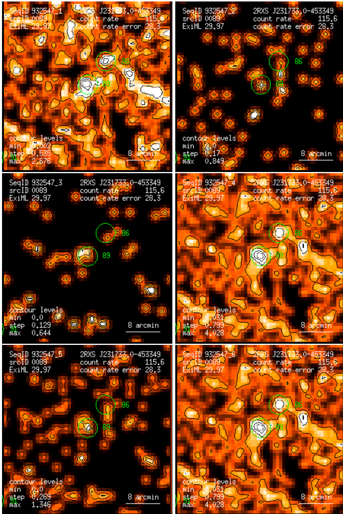
Figure 89: RASS 932547: detection 0089: band rate images, Gaussian filter: (1) PSPC channels 11 – 41, (2) 52 – 90, (3) 91 – 201, (4) 11 – 235, (5) 52 – 201, (6) 11 – 201. Broad band rates in counts/ks. Band rate contour levels in counts/ks/arcmin 2 .
