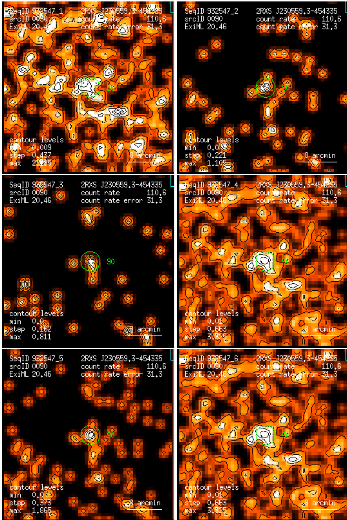
Figure 90: RASS 932547: detection 0090: band rate images, Gaussian filter: (1) PSPC channels 11 – 41, (2) 52 – 90, (3) 91 – 201, (4) 11 – 235, (5) 52 – 201, (6) 11 – 201. Broad band rates in counts/ks. Band rate contour levels in counts/ks/arcmin 2 .
