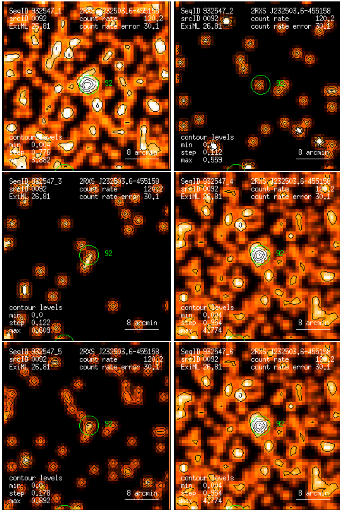
Figure 92: RASS 932547: detection 0092: band rate images, Gaussian filter: (1) PSPC channels 11 – 41, (2) 52 – 90, (3) 91 – 201, (4) 11 – 235, (5) 52 – 201, (6) 11 – 201. Broad band rates in counts/ks. Band rate contour levels in counts/ks/arcmin 2 .
