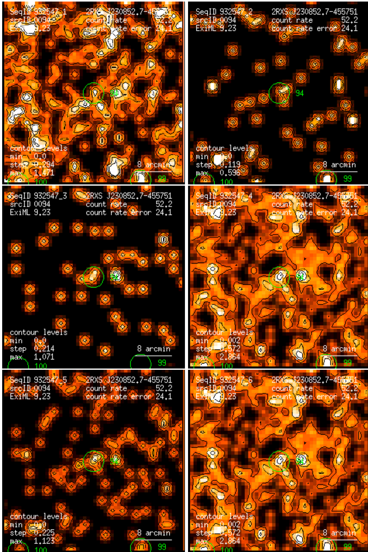
Figure 94: RASS 932547: detection 0094: band rate images, Gaussian filter: (1) PSPC channels 11 – 41, (2) 52 – 90, (3) 91 – 201, (4) 11 – 235, (5) 52 – 201, (6) 11 – 201. Broad band rates in counts/ks. Band rate contour levels in counts/ks/arcmin 2 .
