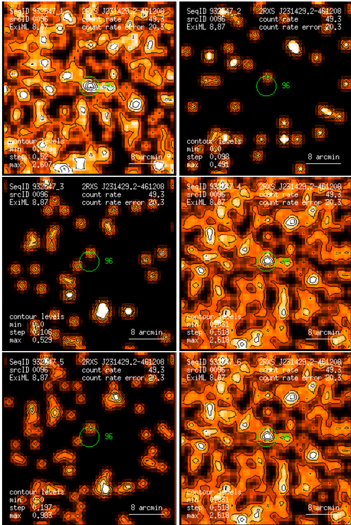
Figure 96: RASS 932547: detection 0096: band rate images, Gaussian filter: (1) PSPC channels 11 – 41, (2) 52 – 90, (3) 91 – 201, (4) 11 – 235, (5) 52 – 201, (6) 11 – 201. Broad band rates in counts/ks. Band rate contour levels in counts/ks/arcmin 2 .
