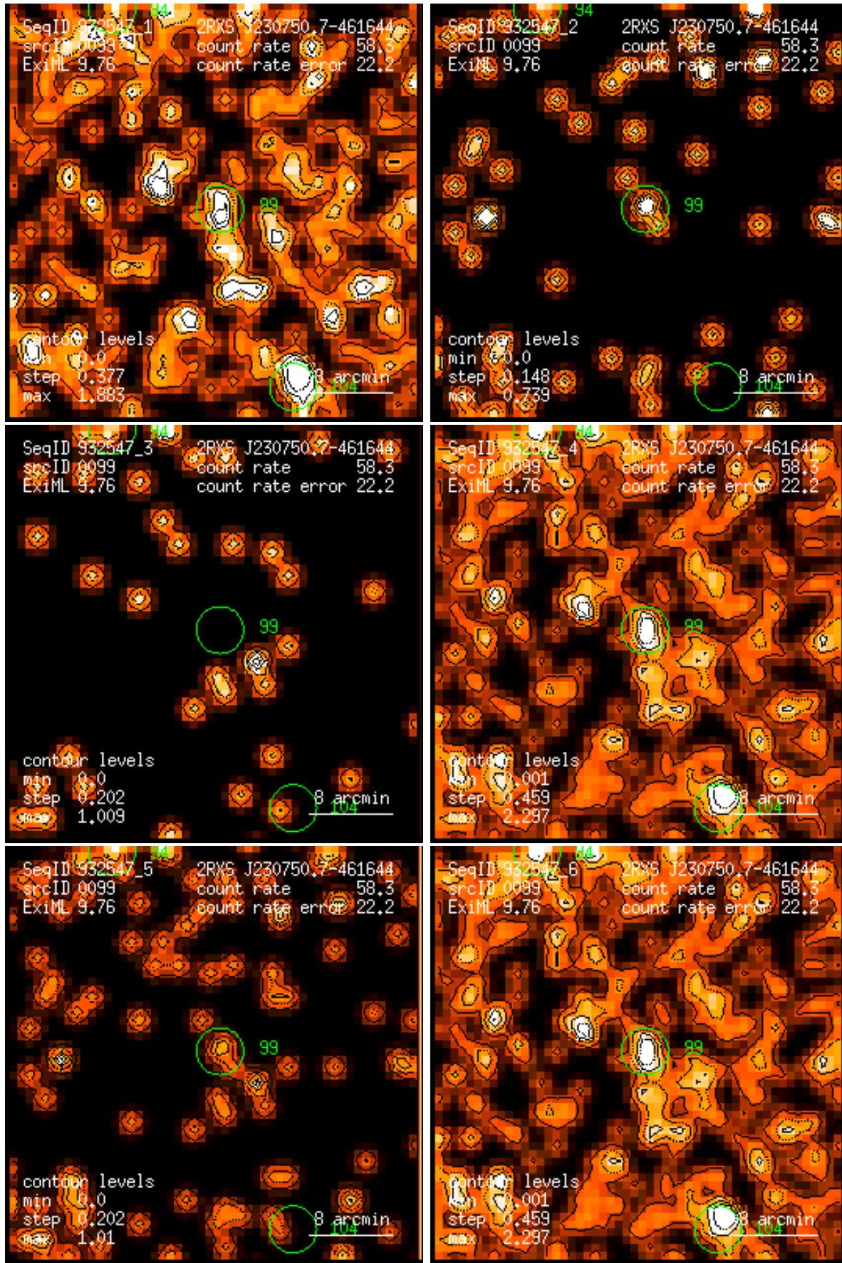
Figure 99: RASS 932547: detection 0099: band rate images, Gaussian filter: (1) PSPC channels 11 – 41, (2) 52 – 90, (3) 91 – 201, (4) 11 – 235, (5) 52 – 201, (6) 11 – 201. Broad band rates in counts/ks. Band rate contour levels in counts/ks/arcmin 2 .
