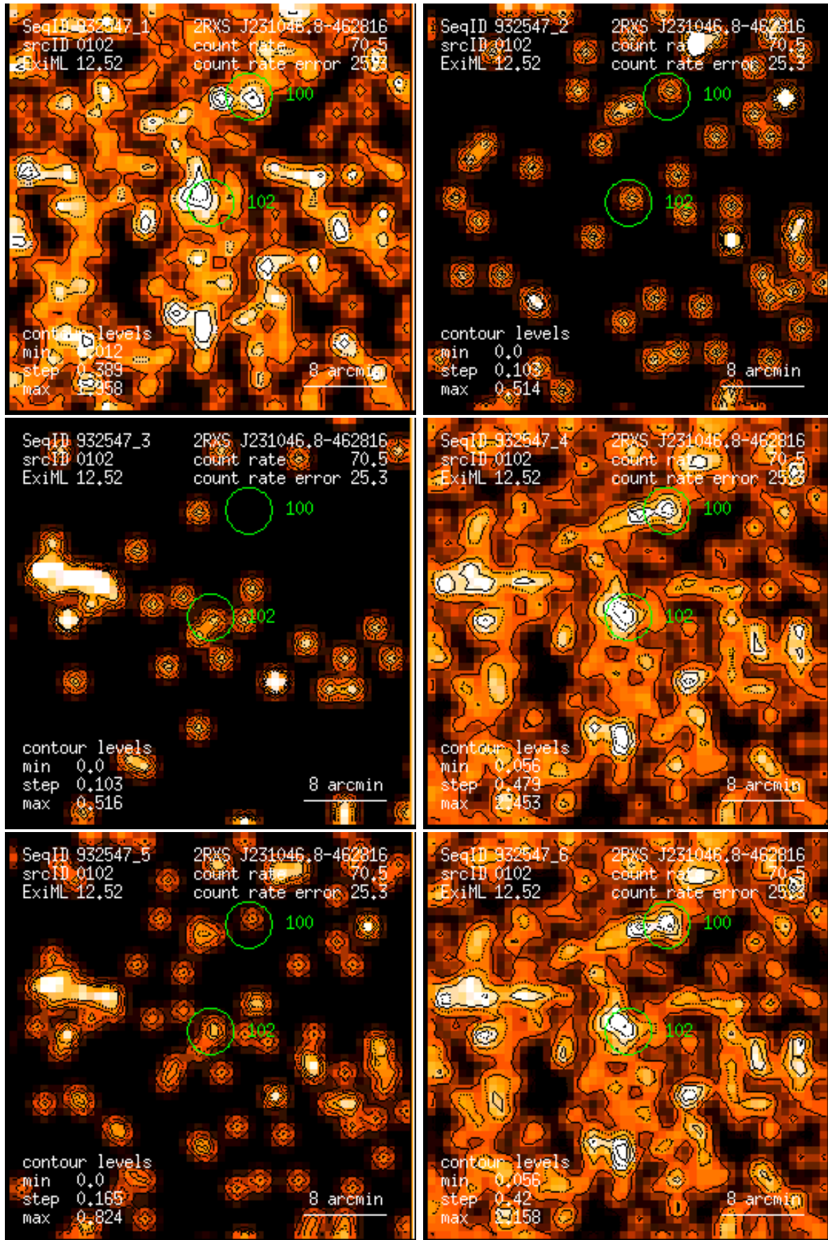
Figure 102: RASS 932547: detection 0102: band rate images, Gaussian filter: (1) PSPC channels 11 – 41, (2) 52 – 90, (3) 91 – 201, (4) 11 – 235, (5) 52 – 201, (6) 11 – 201. Broad band rates in counts/ks. Band rate contour levels in counts/ks/arcmin 2 .
