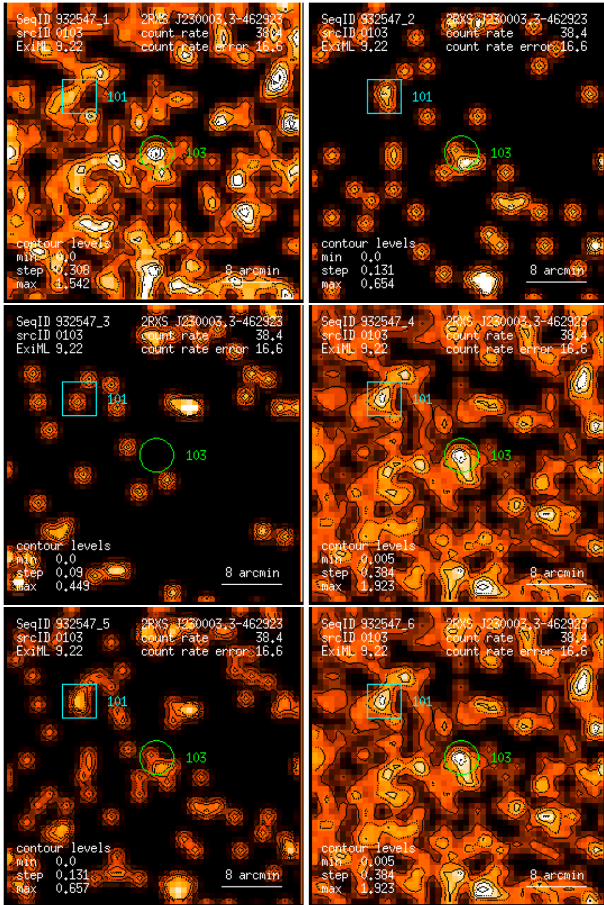
Figure 103: RASS 932547: detection 0103: band rate images, Gaussian filter: (1) PSPC channels 11 – 41, (2) 52 – 90, (3) 91 – 201, (4) 11 – 235, (5) 52 – 201, (6) 11 – 201. Broad band rates in counts/ks. Band rate contour levels in counts/ks/arcmin 2 .
