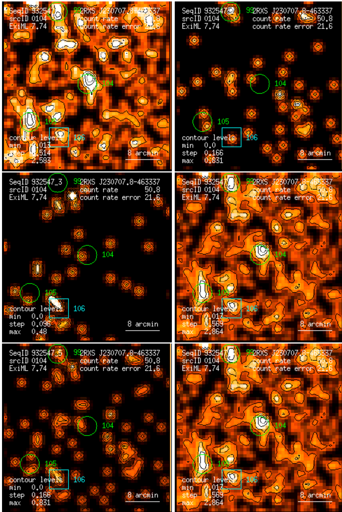
Figure 104: RASS 932547: detection 0104: band rate images, Gaussian filter: (1) PSPC channels 11 – 41, (2) 52 – 90, (3) 91 – 201, (4) 11 – 235, (5) 52 – 201, (6) 11 – 201. Broad band rates in counts/ks. Band rate contour levels in counts/ks/arcmin 2 .
