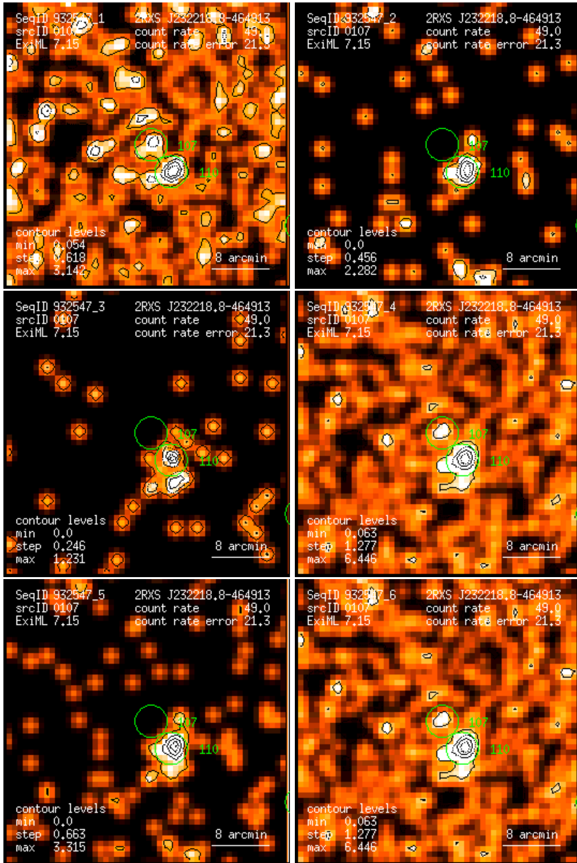
Figure 107: RASS 932547: detection 0107: band rate images, Gaussian filter: (1) PSPC channels 11 – 41, (2) 52 – 90, (3) 91 – 201, (4) 11 – 235, (5) 52 – 201, (6) 11 – 201. Broad band rates in counts/ks. Band rate contour levels in counts/ks/arcmin 2 .
