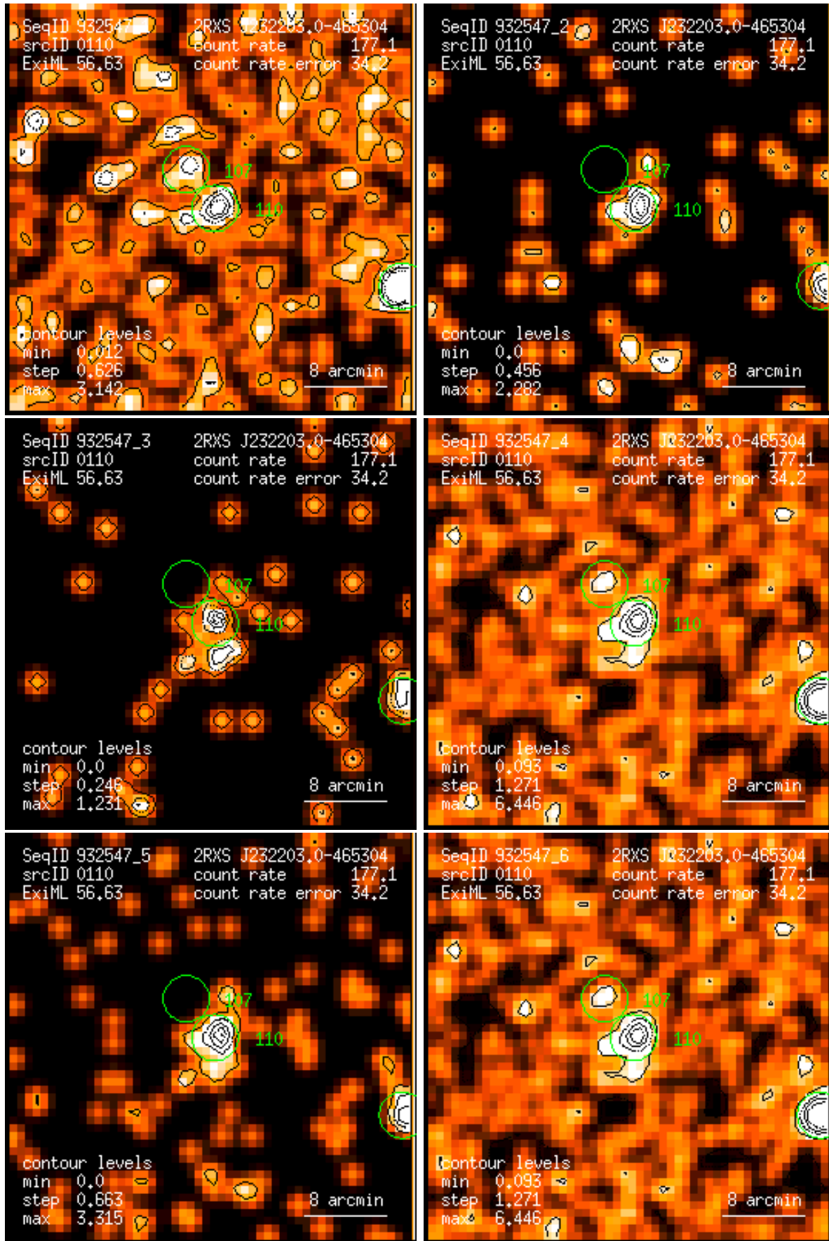
Figure 110: RASS 932547: detection 0110: band rate images, Gaussian filter: (1) PSPC channels 11 – 41, (2) 52 – 90, (3) 91 – 201, (4) 11 – 235, (5) 52 – 201, (6) 11 – 201. Broad band rates in counts/ks. Band rate contour levels in counts/ks/arcmin 2 .
