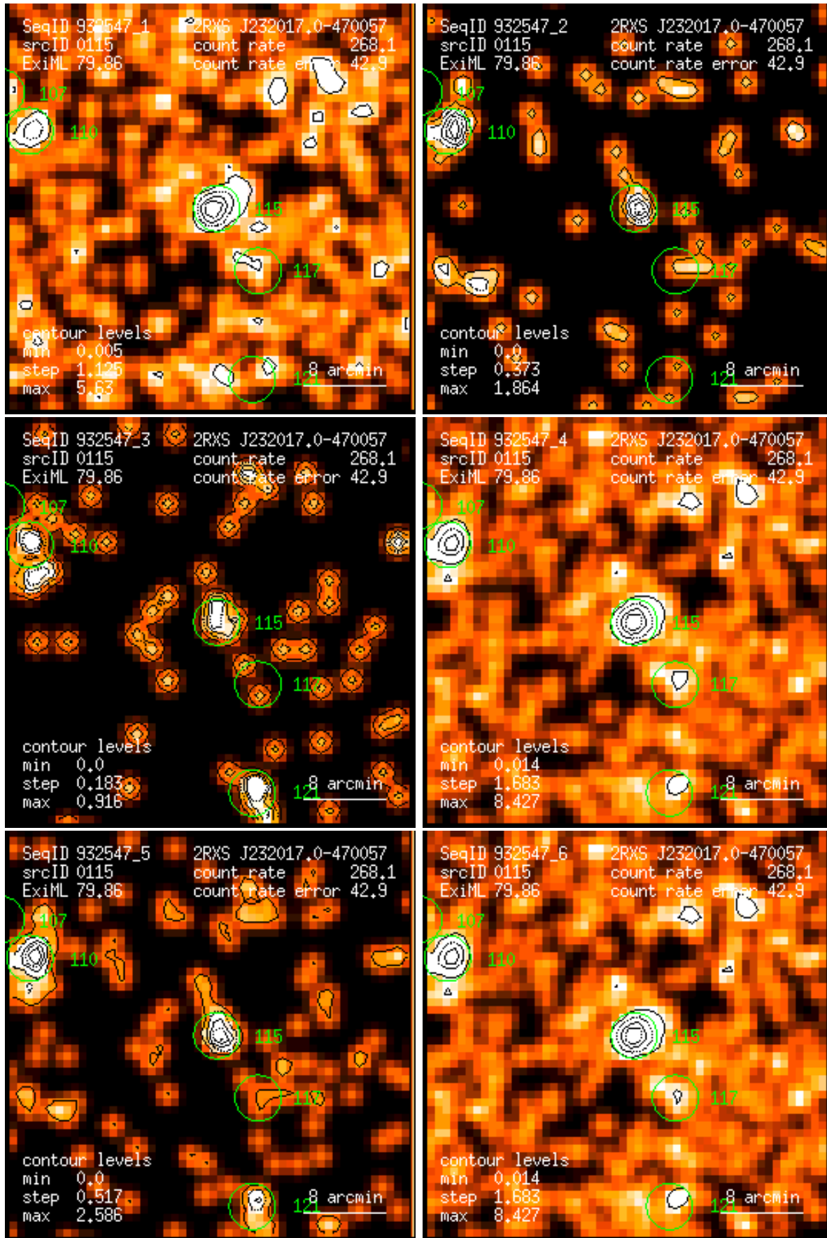
Figure 115: RASS 932547: detection 0115: band rate images, Gaussian filter: (1) PSPC channels 11 – 41, (2) 52 – 90, (3) 91 – 201, (4) 11 – 235, (5) 52 – 201, (6) 11 – 201. Broad band rates in counts/ks. Band rate contour levels in counts/ks/arcmin 2 .
