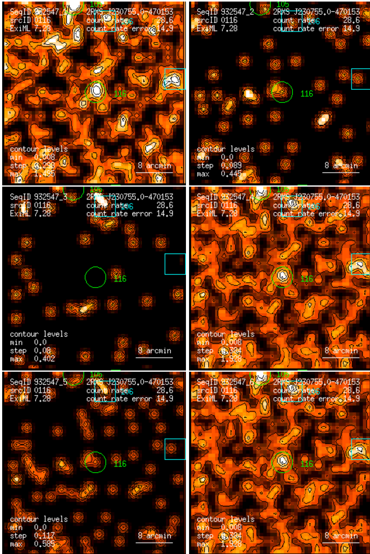
Figure 116: RASS 932547: detection 0116: band rate images, Gaussian filter: (1) PSPC channels 11 – 41, (2) 52 – 90, (3) 91 – 201, (4) 11 – 235, (5) 52 – 201, (6) 11 – 201. Broad band rates in counts/ks. Band rate contour levels in counts/ks/arcmin 2 .
