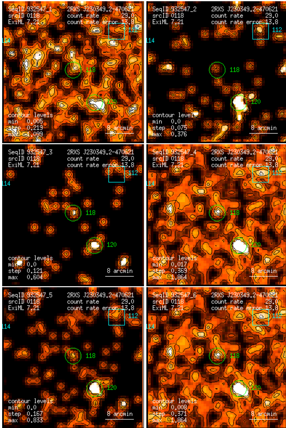
Figure 118: RASS 932547: detection 0118: band rate images, Gaussian filter: (1) PSPC channels 11 – 41, (2) 52 – 90, (3) 91 – 201, (4) 11 – 235, (5) 52 – 201, (6) 11 – 201. Broad band rates in counts/ks. Band rate contour levels in counts/ks/arcmin 2 .
