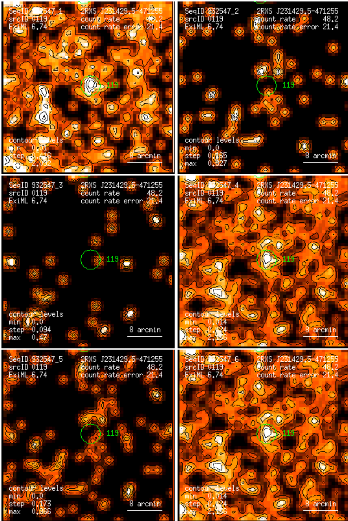
Figure 119: RASS 932547: detection 0119: band rate images, Gaussian filter: (1) PSPC channels 11 – 41, (2) 52 – 90, (3) 91 – 201, (4) 11 – 235, (5) 52 – 201, (6) 11 – 201. Broad band rates in counts/ks. Band rate contour levels in counts/ks/arcmin 2 .
