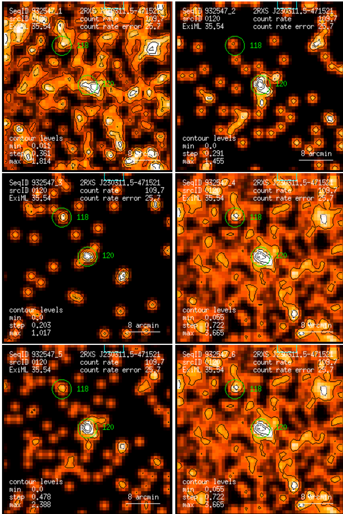
Figure 120: RASS 932547: detection 0120: band rate images, Gaussian filter: (1) PSPC channels 11 – 41, (2) 52 – 90, (3) 91 – 201, (4) 11 – 235, (5) 52 – 201, (6) 11 – 201. Broad band rates in counts/ks. Band rate contour levels in counts/ks/arcmin 2 .
