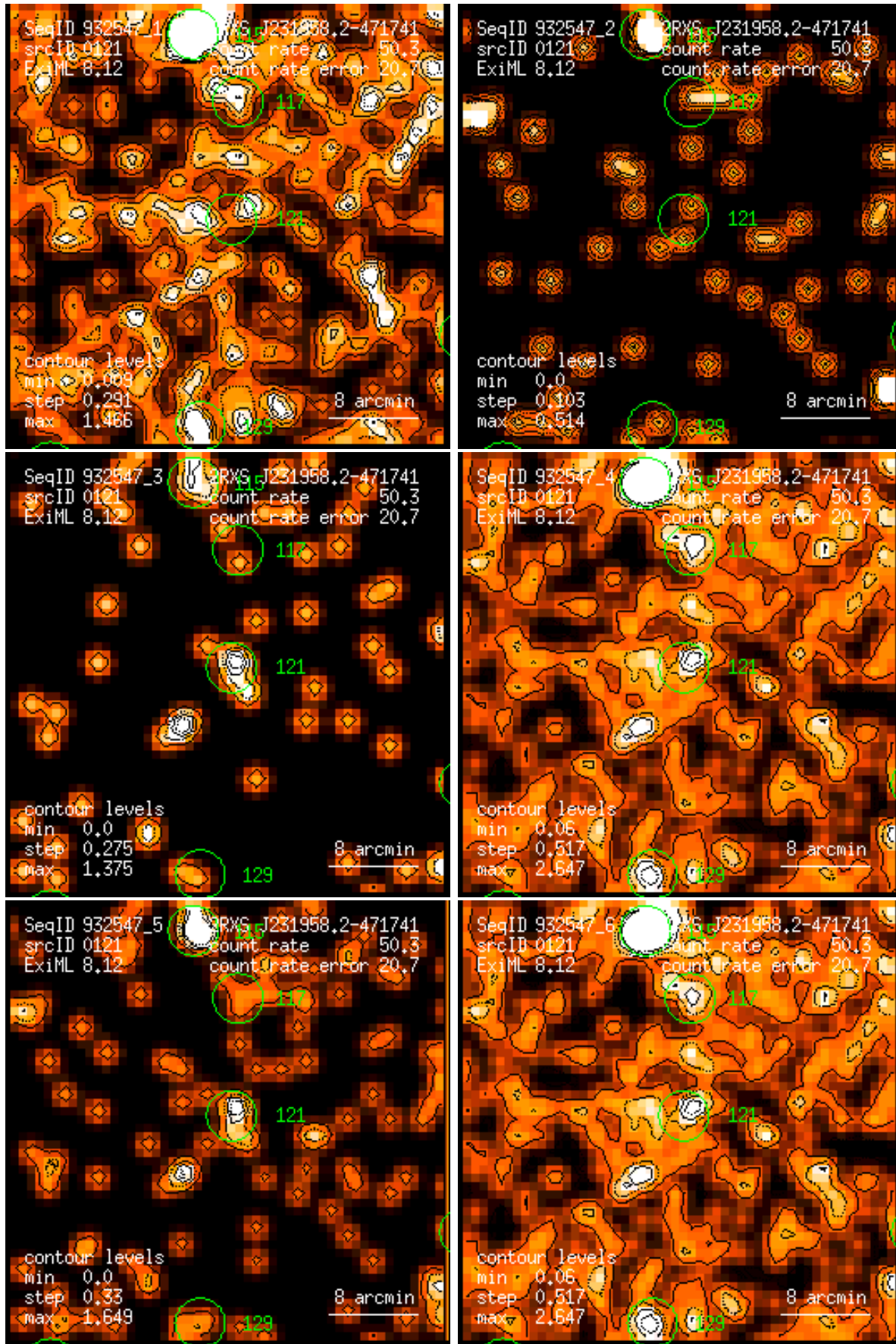
Figure 121: RASS 932547: detection 0121: band rate images, Gaussian filter: (1) PSPC channels 11 – 41, (2) 52 – 90, (3) 91 – 201, (4) 11 – 235, (5) 52 – 201, (6) 11 – 201. Broad band rates in counts/ks. Band rate contour levels in counts/ks/arcmin 2 .
