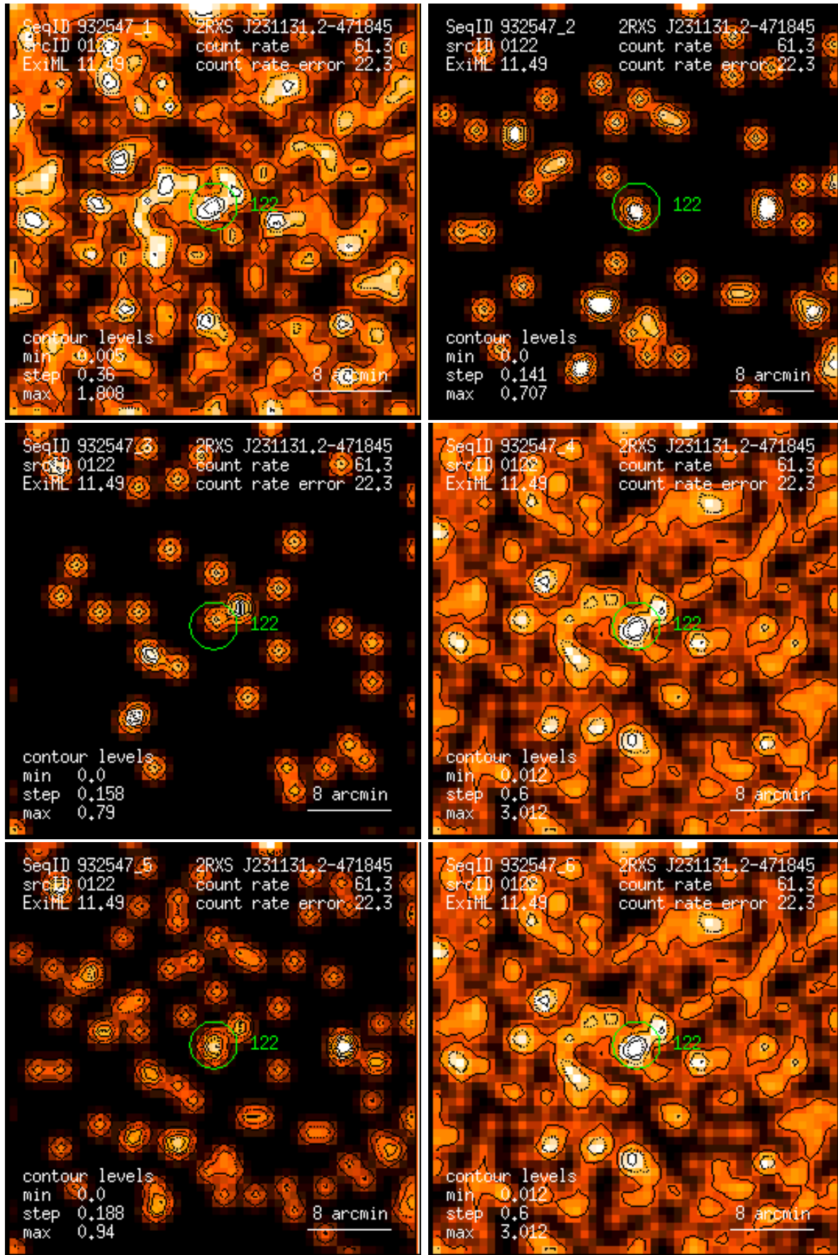
Figure 122: RASS 932547: detection 0122: band rate images, Gaussian filter: (1) PSPC channels 11 – 41, (2) 52 – 90, (3) 91 – 201, (4) 11 – 235, (5) 52 – 201, (6) 11 – 201. Broad band rates in counts/ks. Band rate contour levels in counts/ks/arcmin 2 .
