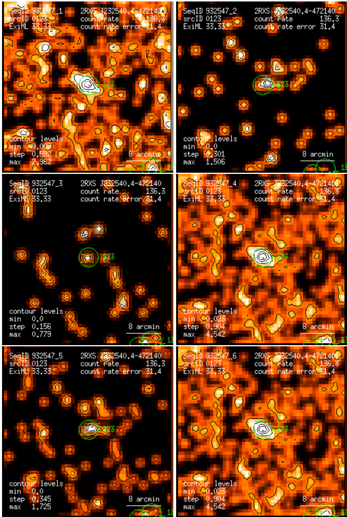
Figure 123: RASS 932547: detection 0123: band rate images, Gaussian filter: (1) PSPC channels 11 – 41, (2) 52 – 90, (3) 91 – 201, (4) 11 – 235, (5) 52 – 201, (6) 11 – 201. Broad band rates in counts/ks. Band rate contour levels in counts/ks/arcmin 2 .
