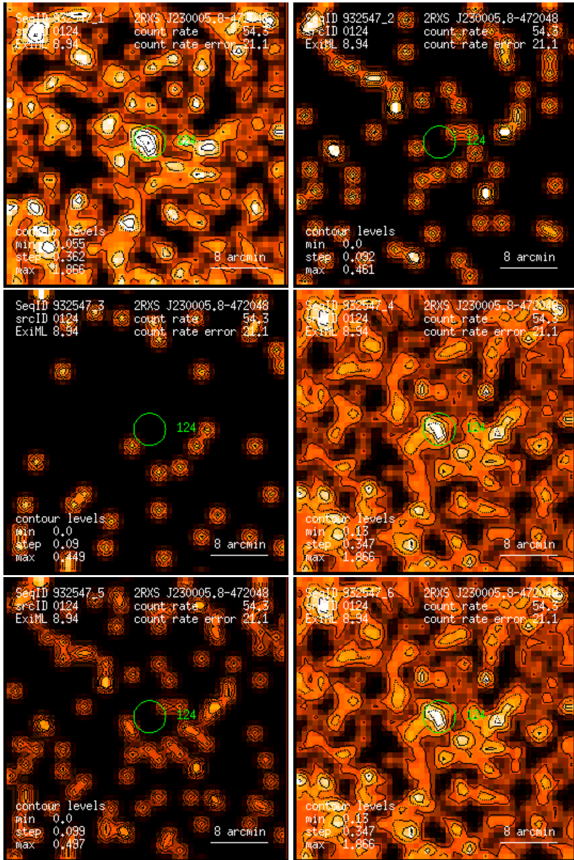
Figure 124: RASS 932547: detection 0124: band rate images, Gaussian filter: (1) PSPC channels 11 – 41, (2) 52 – 90, (3) 91 – 201, (4) 11 – 235, (5) 52 – 201, (6) 11 – 201. Broad band rates in counts/ks. Band rate contour levels in counts/ks/arcmin 2 .
