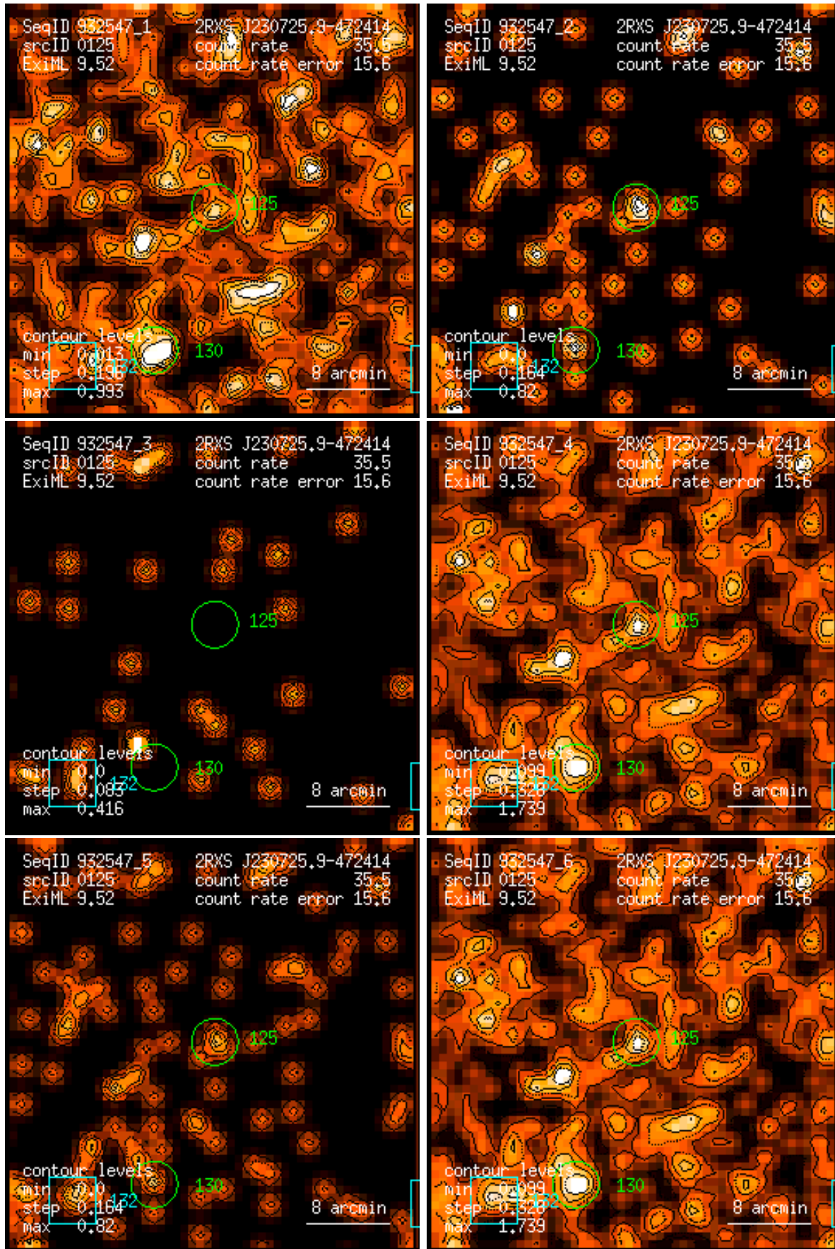
Figure 125: RASS 932547: detection 0125: band rate images, Gaussian filter: (1) PSPC channels 11 – 41, (2) 52 – 90, (3) 91 – 201, (4) 11 – 235, (5) 52 – 201, (6) 11 – 201. Broad band rates in counts/ks. Band rate contour levels in counts/ks/arcmin 2 .
