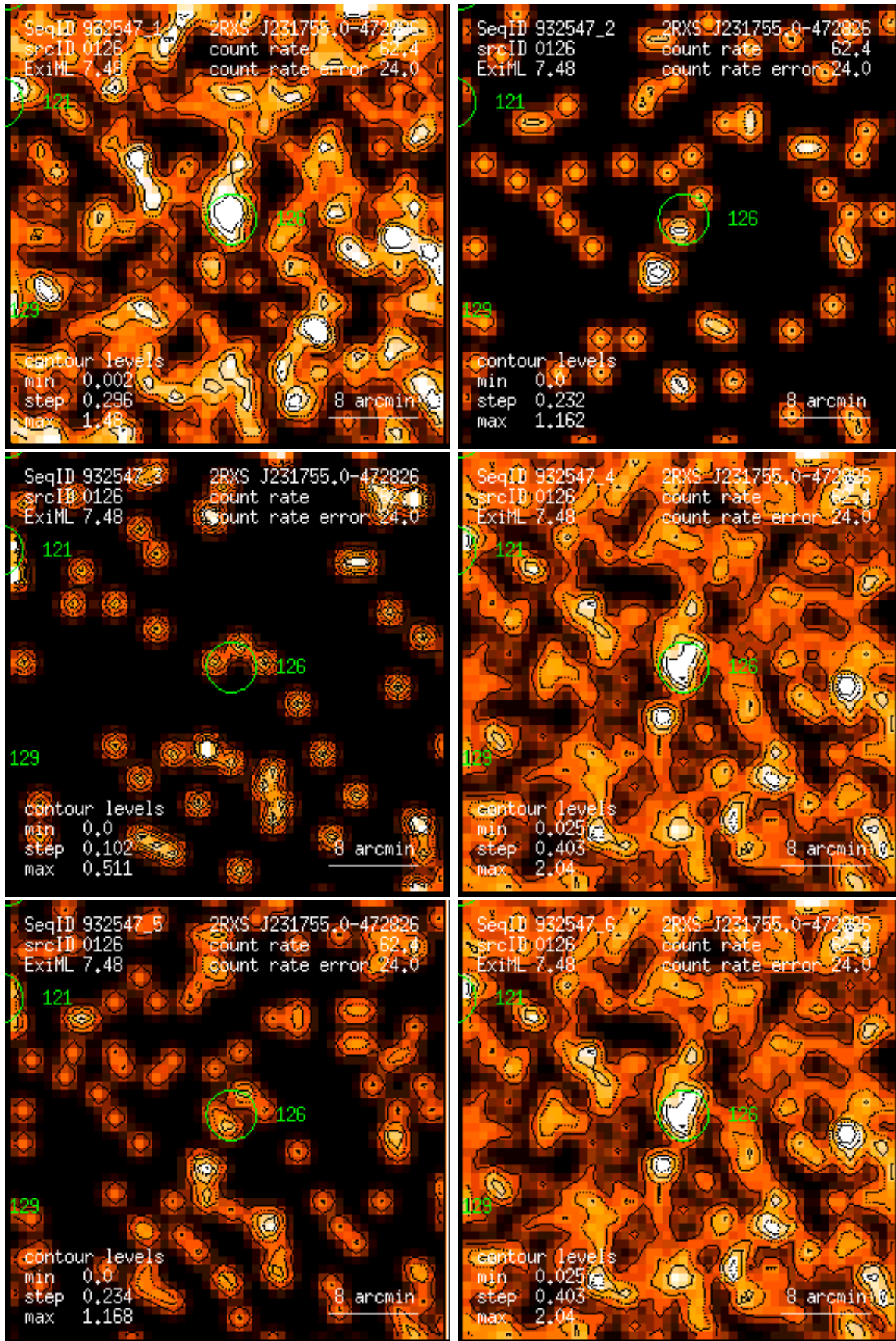
Figure 126: RASS 932547: detection 0126: band rate images, Gaussian filter: (1) PSPC channels 11 – 41, (2) 52 – 90, (3) 91 – 201, (4) 11 – 235, (5) 52 – 201, (6) 11 – 201. Broad band rates in counts/ks. Band rate contour levels in counts/ks/arcmin 2 .
