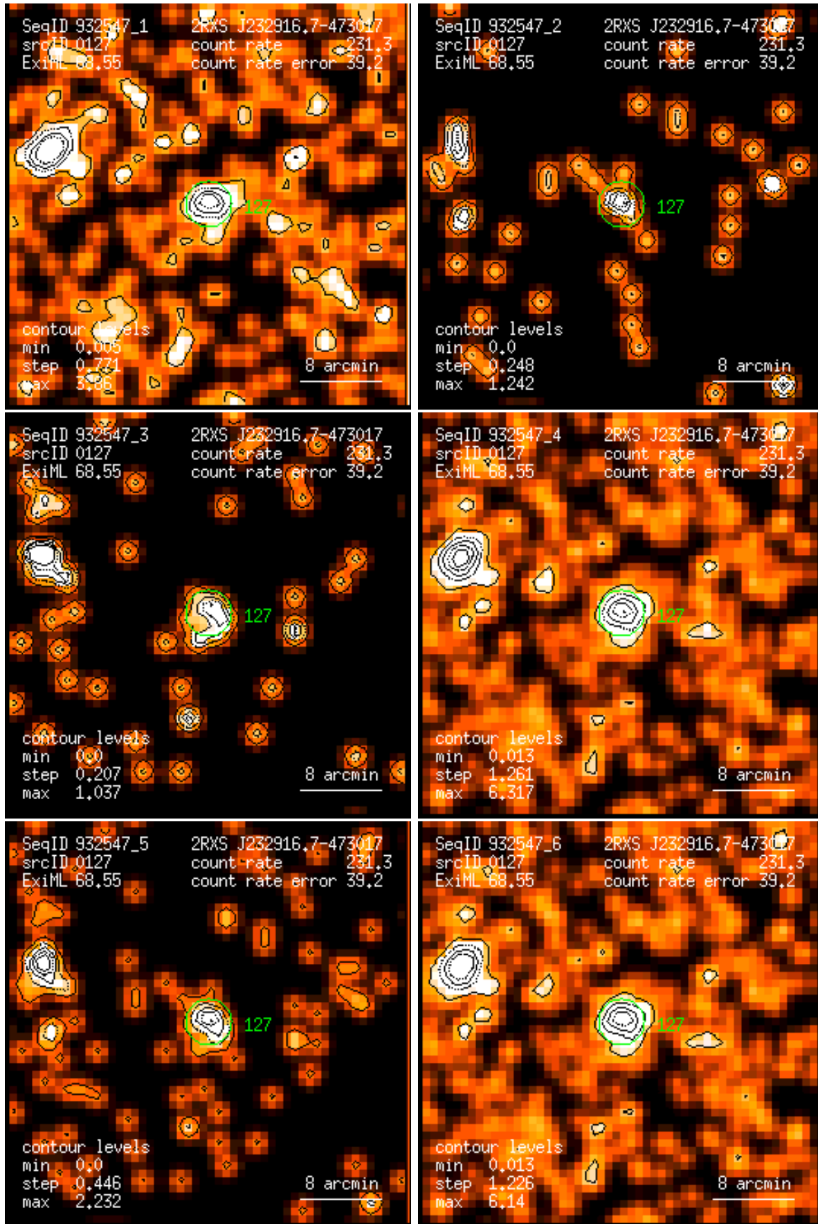
Figure 127: RASS 932547: detection 0127: band rate images, Gaussian filter: (1) PSPC channels 11 – 41, (2) 52 – 90, (3) 91 – 201, (4) 11 – 235, (5) 52 – 201, (6) 11 – 201. Broad band rates in counts/ks. Band rate contour levels in counts/ks/arcmin 2 .
