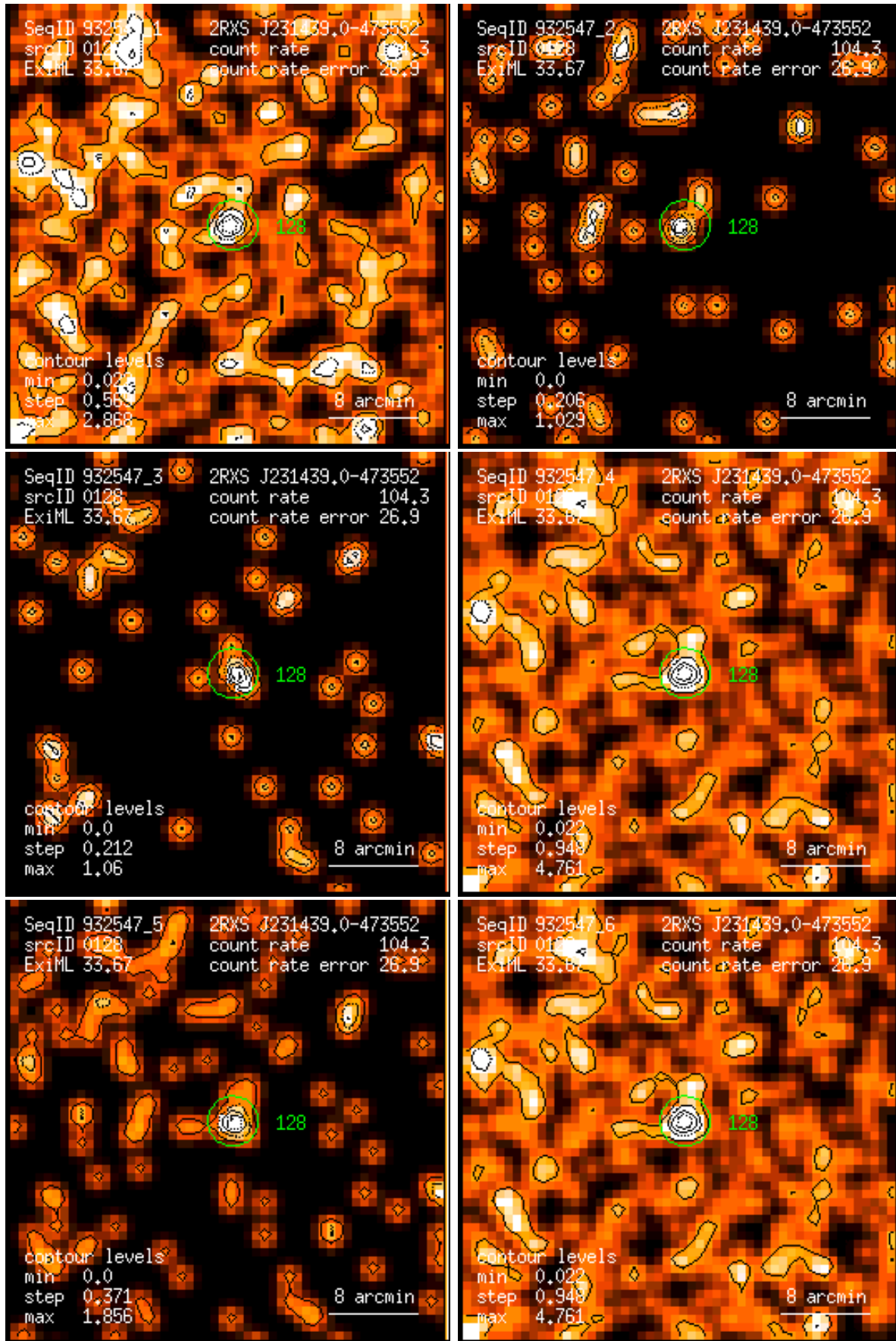
Figure 128: RASS 932547: detection 0128: band rate images, Gaussian filter: (1) PSPC channels 11 – 41, (2) 52 – 90, (3) 91 – 201, (4) 11 – 235, (5) 52 – 201, (6) 11 – 201. Broad band rates in counts/ks. Band rate contour levels in counts/ks/arcmin 2 .
