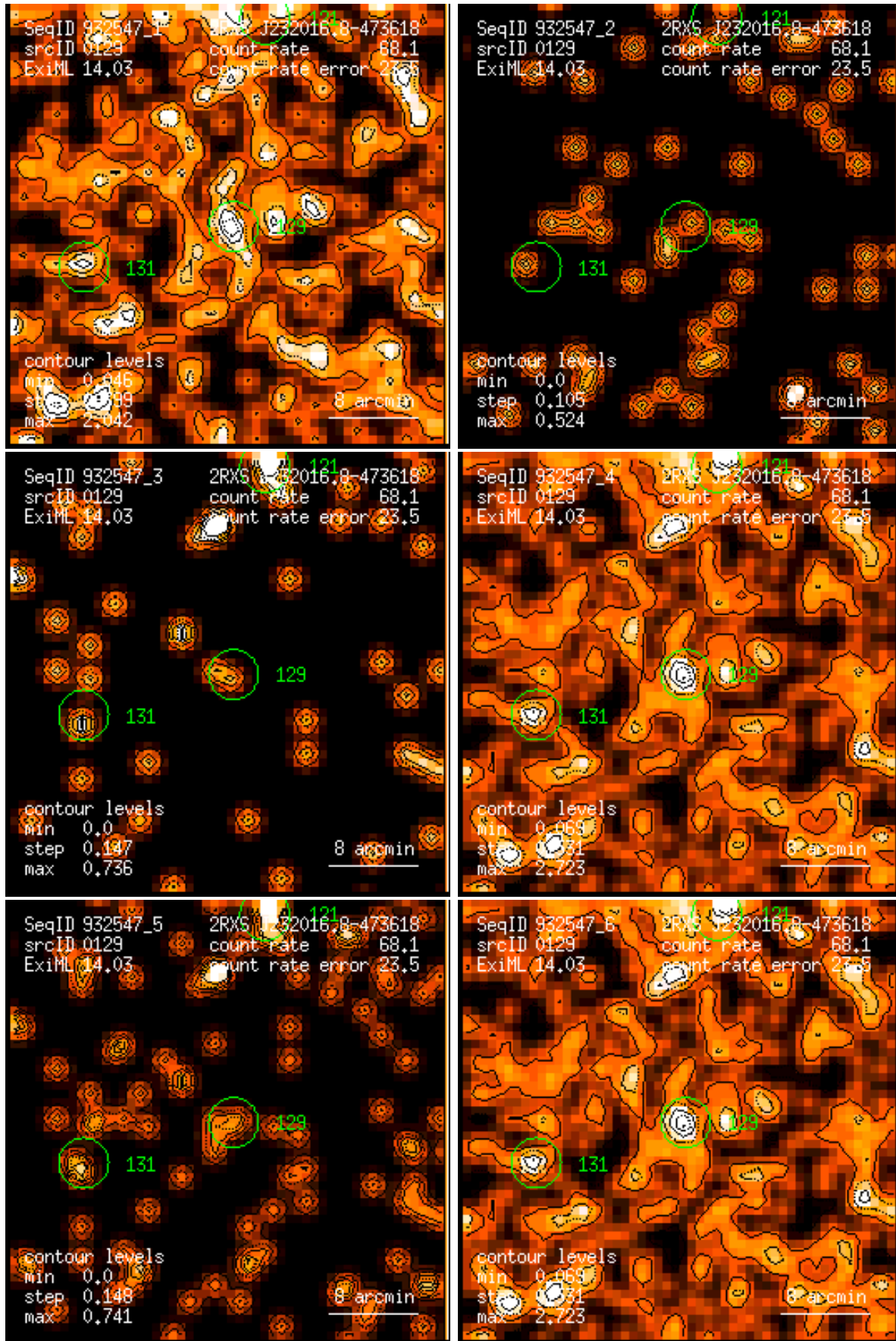
Figure 129: RASS 932547: detection 0129: band rate images, Gaussian filter: (1) PSPC channels 11 – 41, (2) 52 – 90, (3) 91 – 201, (4) 11 – 235, (5) 52 – 201, (6) 11 – 201. Broad band rates in counts/ks. Band rate contour levels in counts/ks/arcmin 2 .
