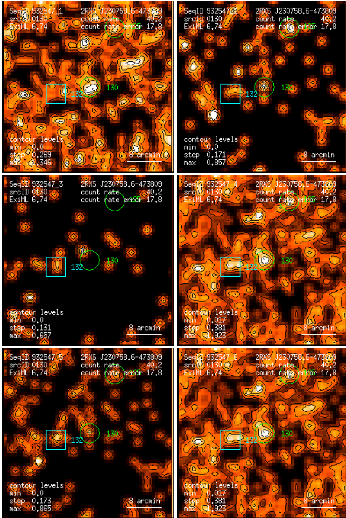
Figure 130: RASS 932547: detection 0130: band rate images, Gaussian filter: (1) PSPC channels 11 – 41, (2) 52 – 90, (3) 91 – 201, (4) 11 – 235, (5) 52 – 201, (6) 11 – 201. Broad band rates in counts/ks. Band rate contour levels in counts/ks/arcmin 2 .
