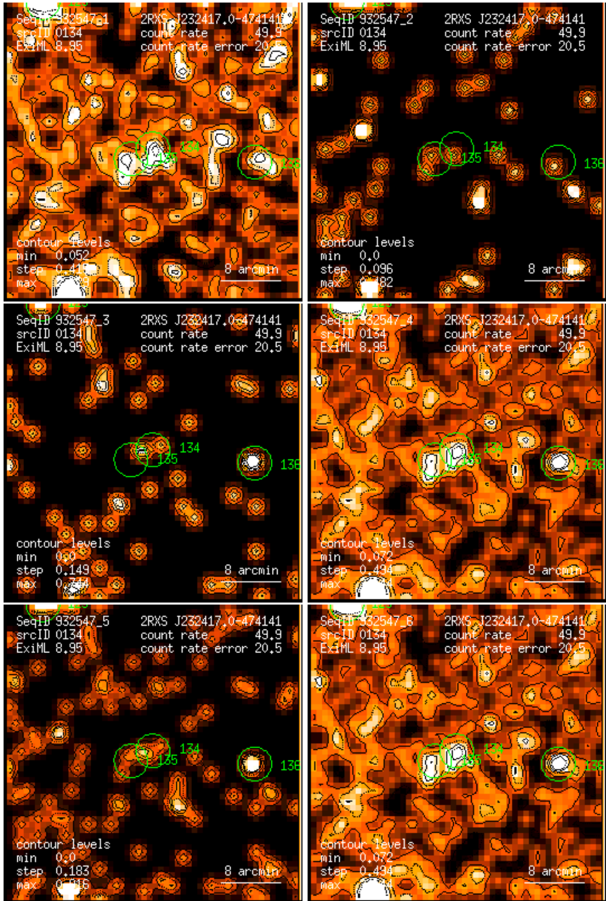
Figure 134: RASS 932547: detection 0134: band rate images, Gaussian filter: (1) PSPC channels 11 – 41, (2) 52 – 90, (3) 91 – 201, (4) 11 – 235, (5) 52 – 201, (6) 11 – 201. Broad band rates in counts/ks. Band rate contour levels in counts/ks/arcmin 2 .
