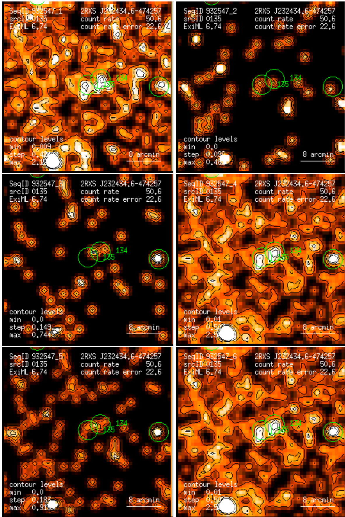
Figure 135: RASS 932547: detection 0135: band rate images, Gaussian filter: (1) PSPC channels 11 – 41, (2) 52 – 90, (3) 91 – 201, (4) 11 – 235, (5) 52 – 201, (6) 11 – 201. Broad band rates in counts/ks. Band rate contour levels in counts/ks/arcmin 2 .
