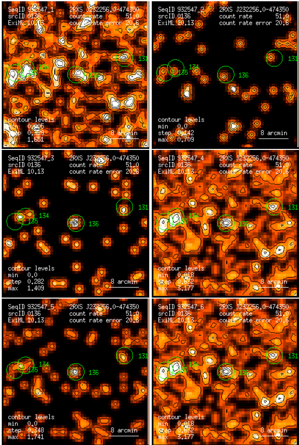
Figure 136: RASS 932547: detection 0136: band rate images, Gaussian filter: (1) PSPC channels 11 – 41, (2) 52 – 90, (3) 91 – 201, (4) 11 – 235, (5) 52 – 201, (6) 11 – 201. Broad band rates in counts/ks. Band rate contour levels in counts/ks/arcmin 2 .
