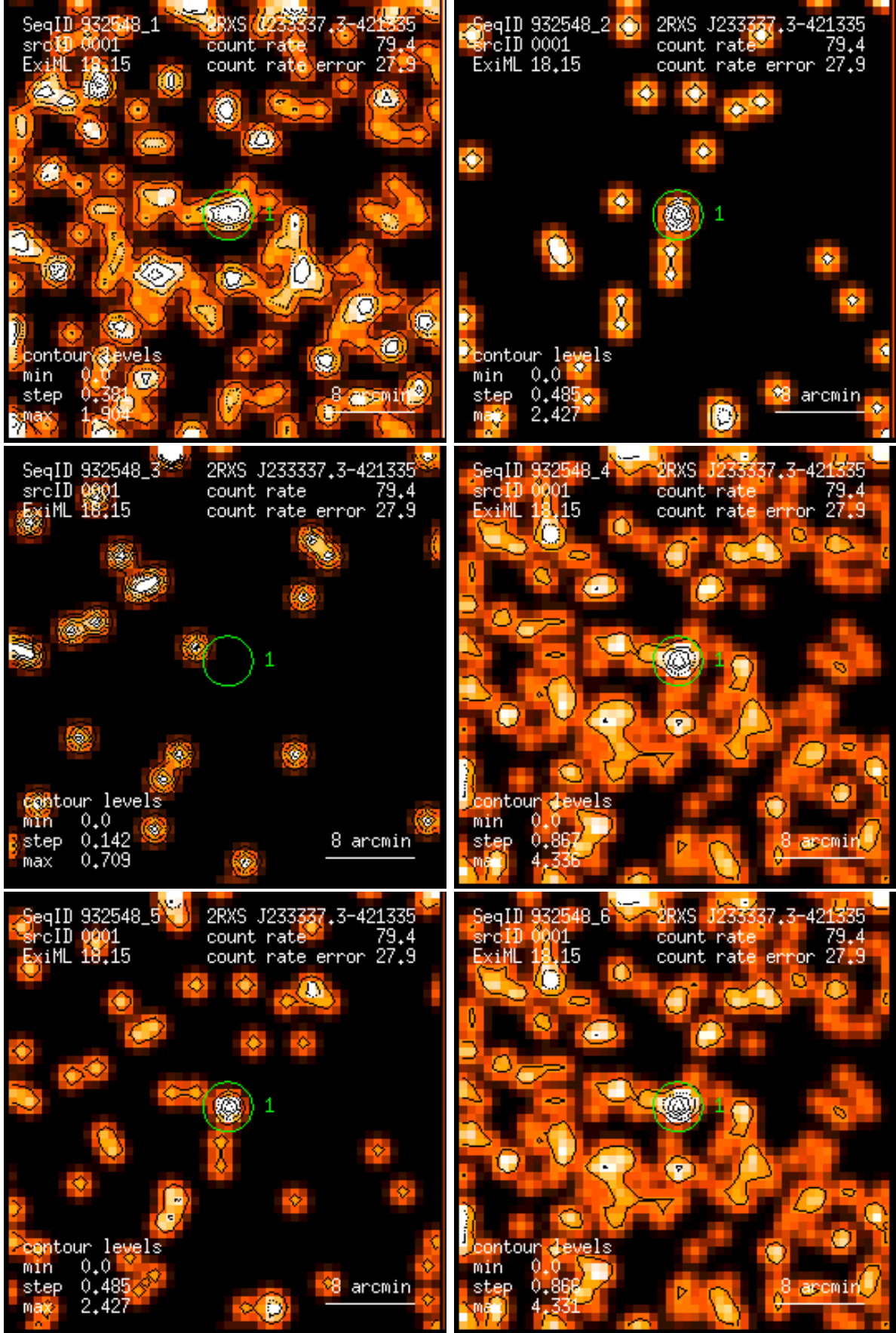
Figure 1: RASS 932548: detection 0001: band rate images, Gaussian filter: (1) PSPC channels 11 – 41, (2) 52 – 90, (3) 91 – 201, (4) 11 – 235, (5) 52 – 201, (6) 11 – 201. Broad band rates in counts/ks. Band rate contour levels in counts/ks/arcmin 2 .
