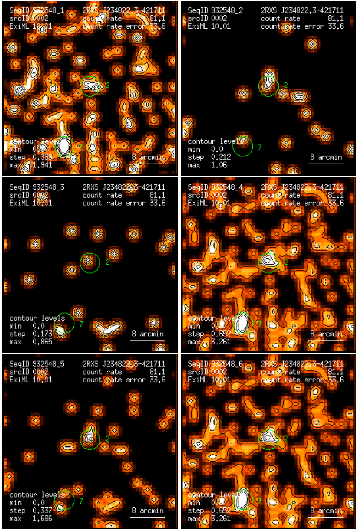
Figure 2: RASS 932548: detection 0002: band rate images, Gaussian filter: (1) PSPC channels 11 – 41, (2) 52 – 90, (3) 91 – 201, (4) 11 – 235, (5) 52 – 201, (6) 11 – 201. Broad band rates in counts/ks. Band rate contour levels in counts/ks/arcmin 2 .
