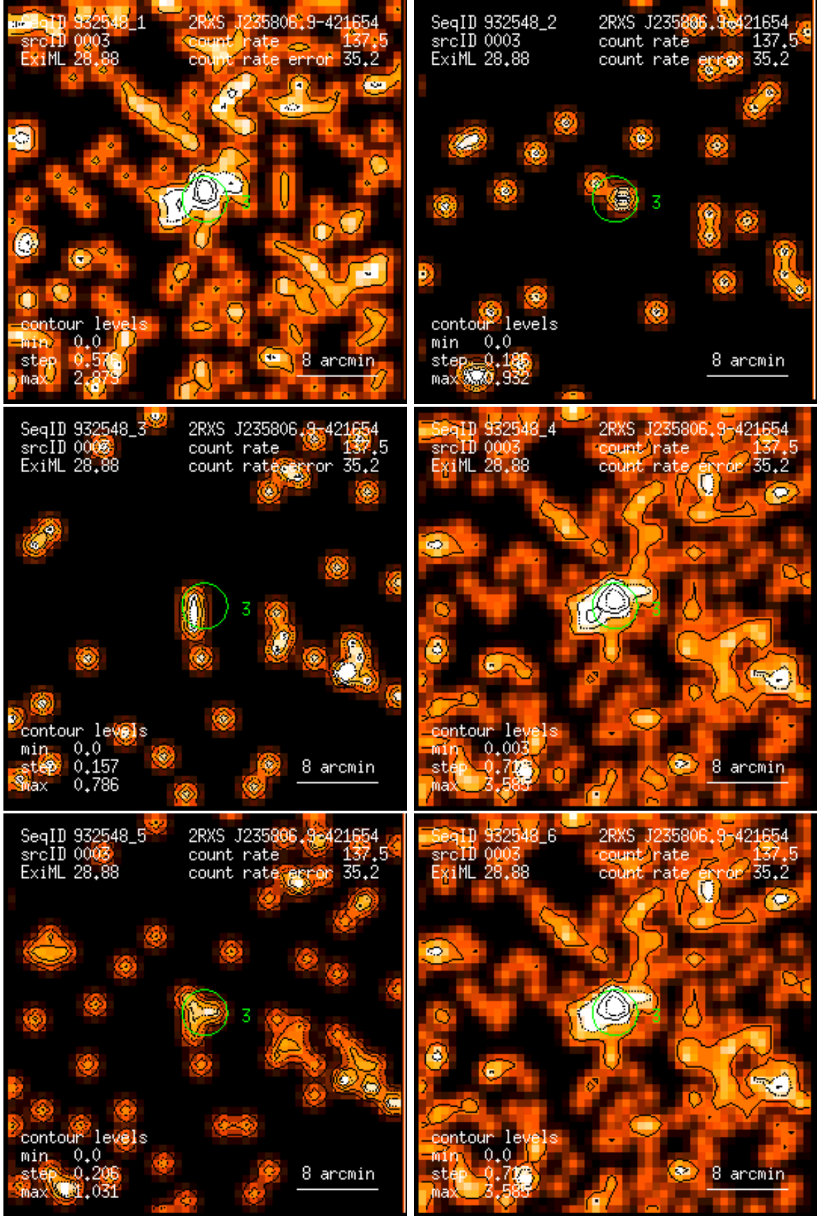
Figure 3: RASS 932548: detection 0003: band rate images, Gaussian filter: (1) PSPC channels 11 – 41, (2) 52 – 90, (3) 91 – 201, (4) 11 – 235, (5) 52 – 201, (6) 11 – 201. Broad band rates in counts/ks. Band rate contour levels in counts/ks/arcmin 2 .
