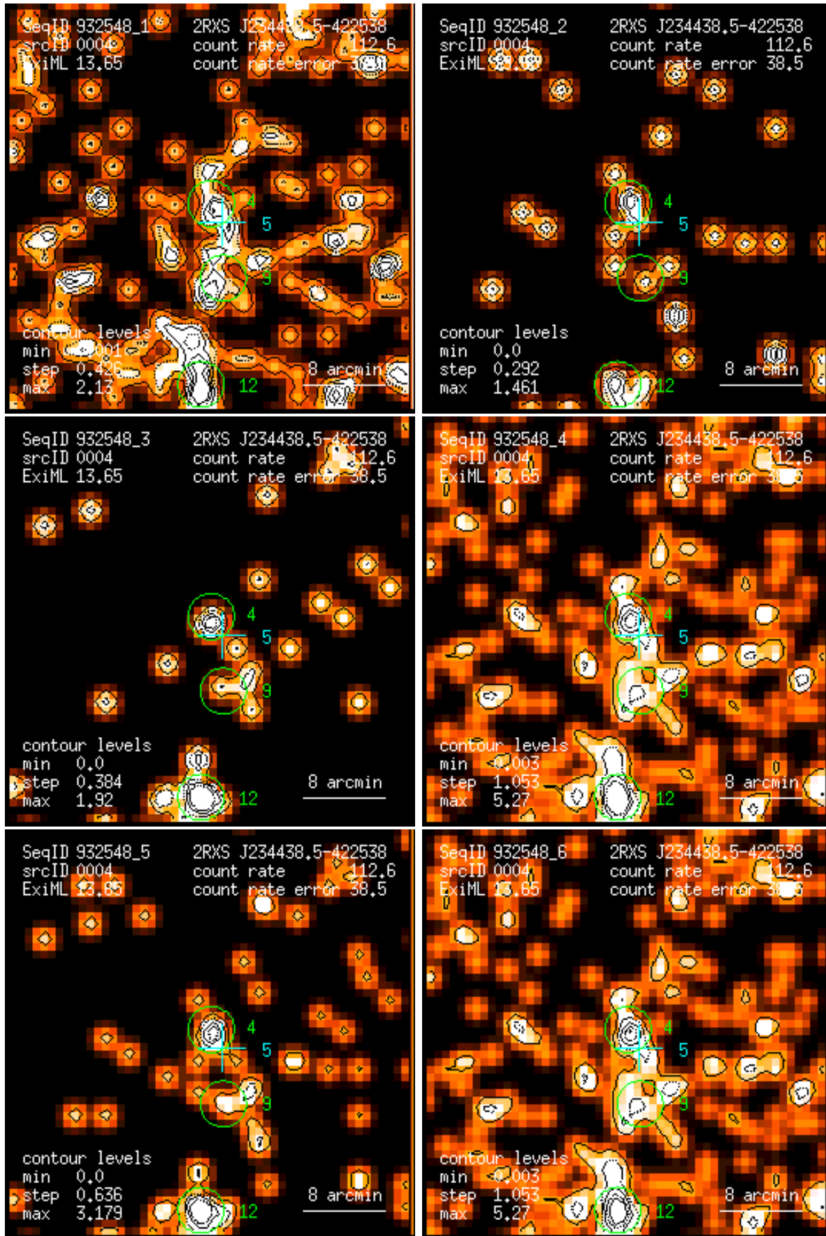
Figure 4: RASS 932548: detection 0004: band rate images, Gaussian filter: (1) PSPC channels 11 – 41, (2) 52 – 90, (3) 91 – 201, (4) 11 – 235, (5) 52 – 201, (6) 11 – 201. Broad band rates in counts/ks. Band rate contour levels in counts/ks/arcmin 2 .
