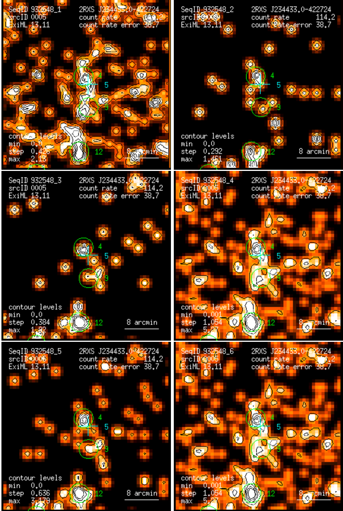
Figure 5: RASS 932548: detection 0005: band rate images, Gaussian filter: (1) PSPC channels 11 – 41, (2) 52 – 90, (3) 91 – 201, (4) 11 – 235, (5) 52 – 201, (6) 11 – 201. Broad band rates in counts/ks. Band rate contour levels in counts/ks/arcmin 2 .
