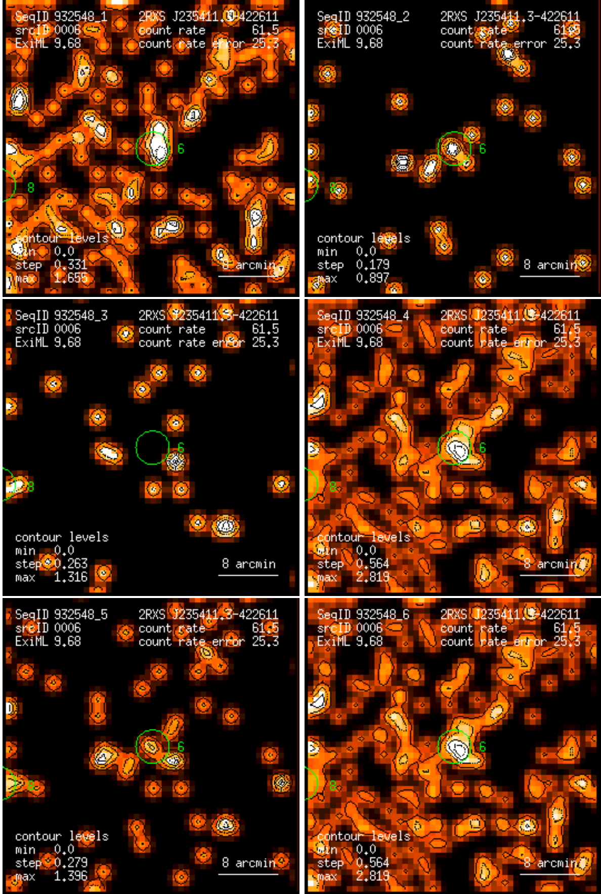
Figure 6: RASS 932548: detection 0006: band rate images, Gaussian filter: (1) PSPC channels 11 – 41, (2) 52 – 90, (3) 91 – 201, (4) 11 – 235, (5) 52 – 201, (6) 11 – 201. Broad band rates in counts/ks. Band rate contour levels in counts/ks/arcmin 2 .
