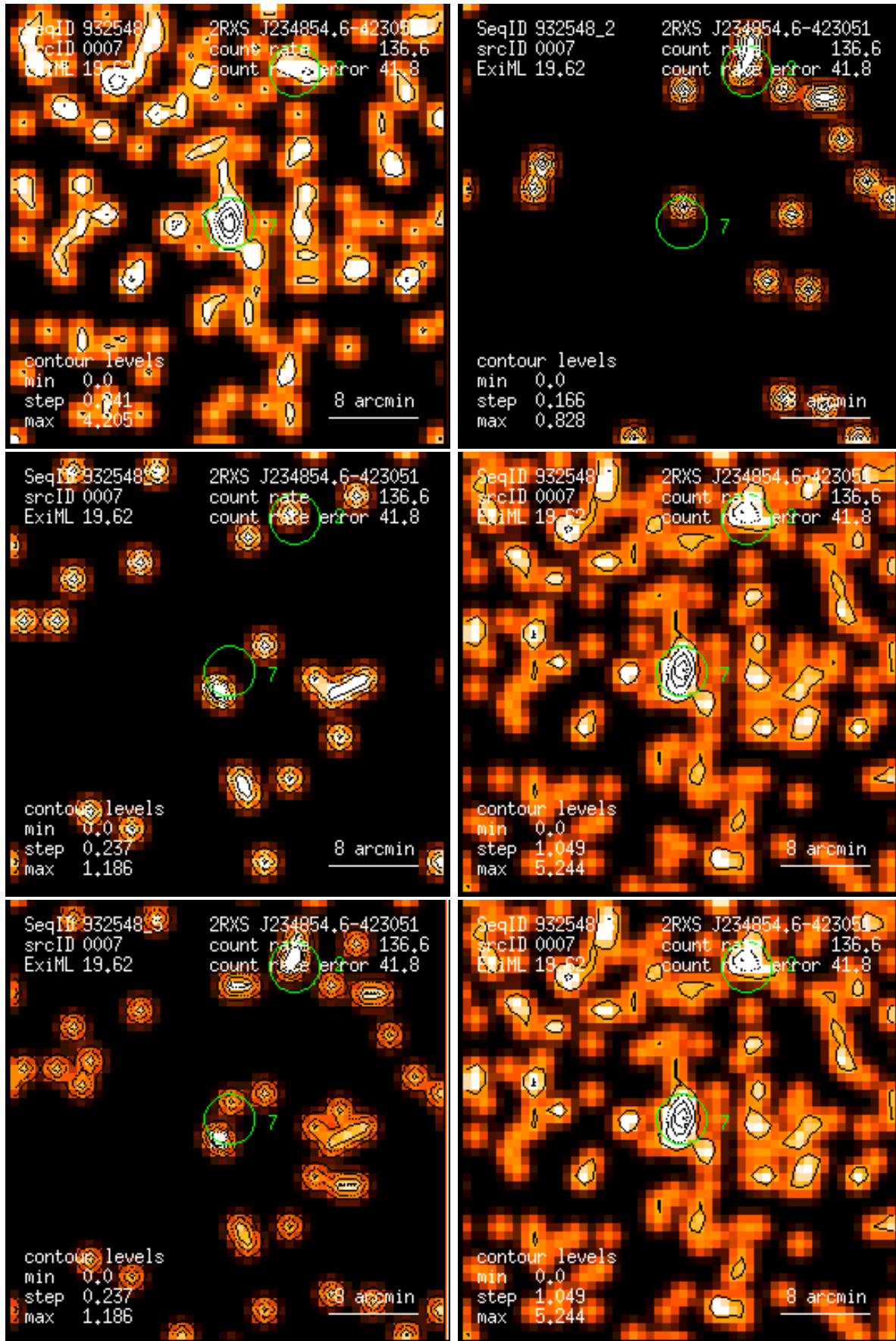
Figure 7: RASS 932548: detection 0007: band rate images, Gaussian filter: (1) PSPC channels 11 – 41, (2) 52 – 90, (3) 91 – 201, (4) 11 – 235, (5) 52 – 201, (6) 11 – 201. Broad band rates in counts/ks. Band rate contour levels in counts/ks/arcmin 2 .
