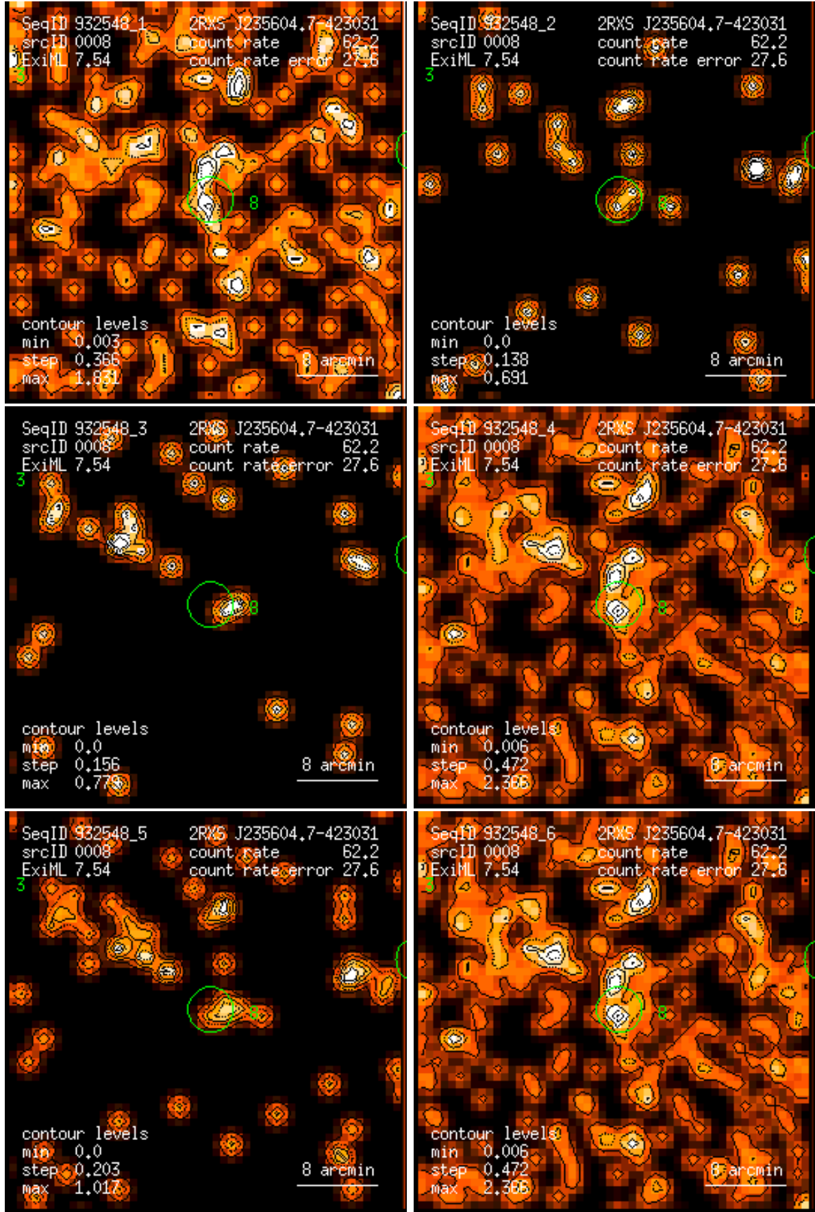
Figure 8: RASS 932548: detection 0008: band rate images, Gaussian filter: (1) PSPC channels 11 – 41, (2) 52 – 90, (3) 91 – 201, (4) 11 – 235, (5) 52 – 201, (6) 11 – 201. Broad band rates in counts/ks. Band rate contour levels in counts/ks/arcmin 2 .
