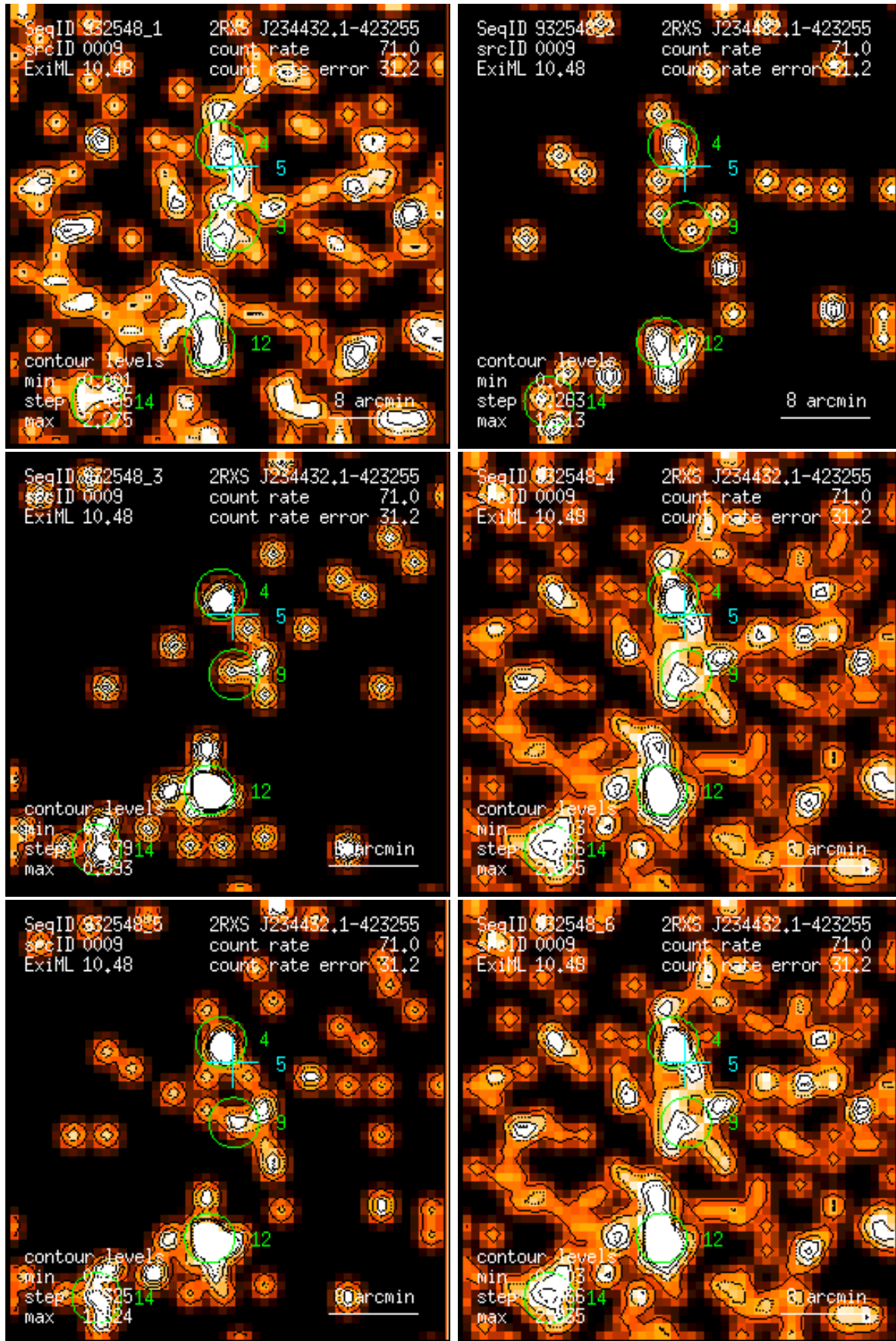
Figure 9: RASS 932548: detection 0009: band rate images, Gaussian filter: (1) PSPC channels 11 – 41, (2) 52 – 90, (3) 91 – 201, (4) 11 – 235, (5) 52 – 201, (6) 11 – 201. Broad band rates in counts/ks. Band rate contour levels in counts/ks/arcmin 2 .
