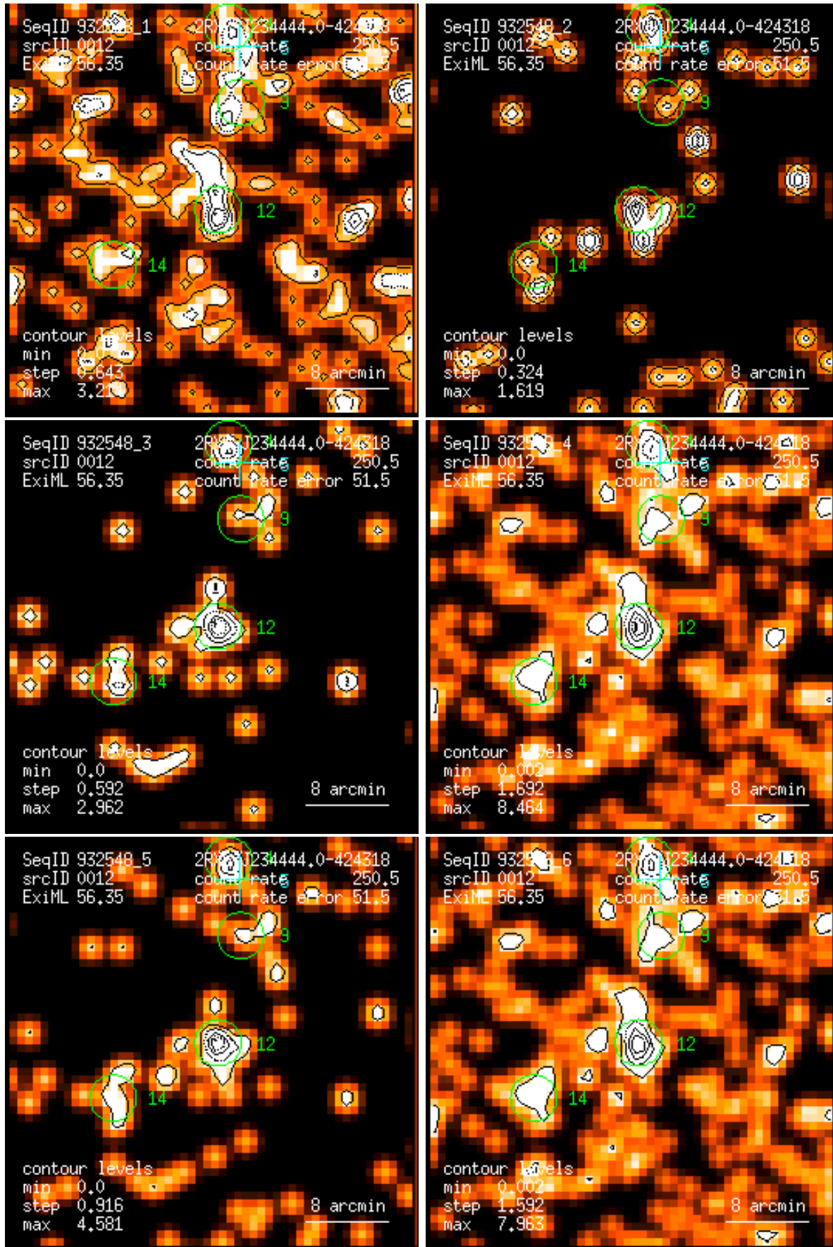
Figure 12: RASS 932548: detection 0012: band rate images, Gaussian filter: (1) PSPC channels 11 – 41, (2) 52 – 90, (3) 91 – 201, (4) 11 – 235, (5) 52 – 201, (6) 11 – 201. Broad band rates in counts/ks. Band rate contour levels in counts/ks/arcmin 2 .
