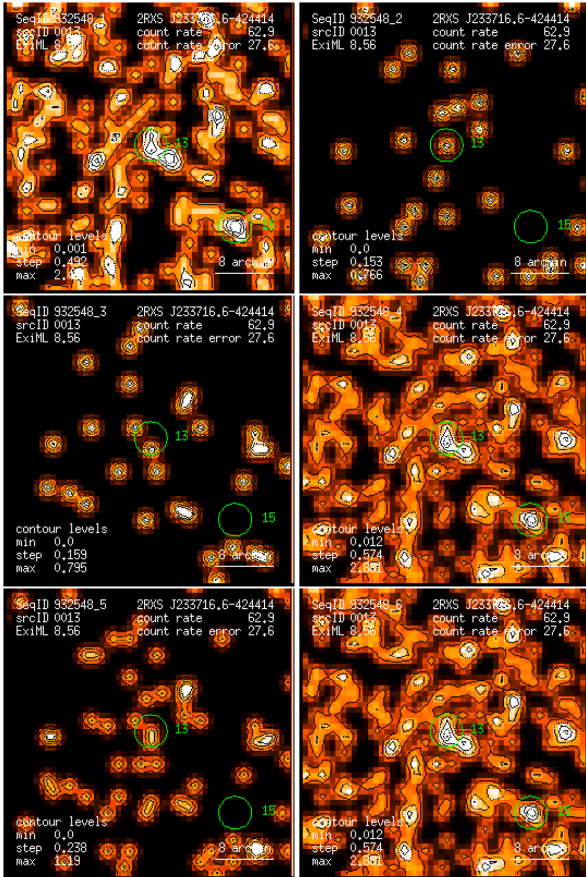
Figure 13: RASS 932548: detection 0013: band rate images, Gaussian filter: (1) PSPC channels 11 – 41, (2) 52 – 90, (3) 91 – 201, (4) 11 – 235, (5) 52 – 201, (6) 11 – 201. Broad band rates in counts/ks. Band rate contour levels in counts/ks/arcmin 2 .
