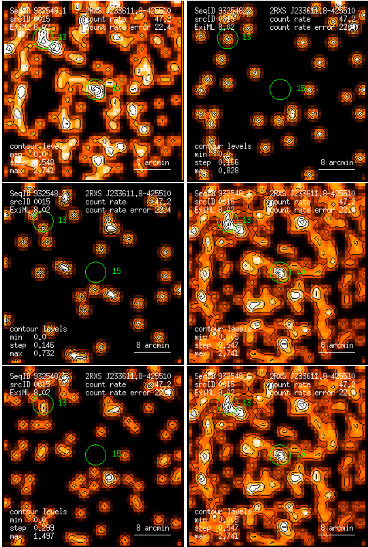
Figure 15: RASS 932548: detection 0015: band rate images, Gaussian filter: (1) PSPC channels 11 – 41, (2) 52 – 90, (3) 91 – 201, (4) 11 – 235, (5) 52 – 201, (6) 11 – 201. Broad band rates in counts/ks. Band rate contour levels in counts/ks/arcmin 2 .
