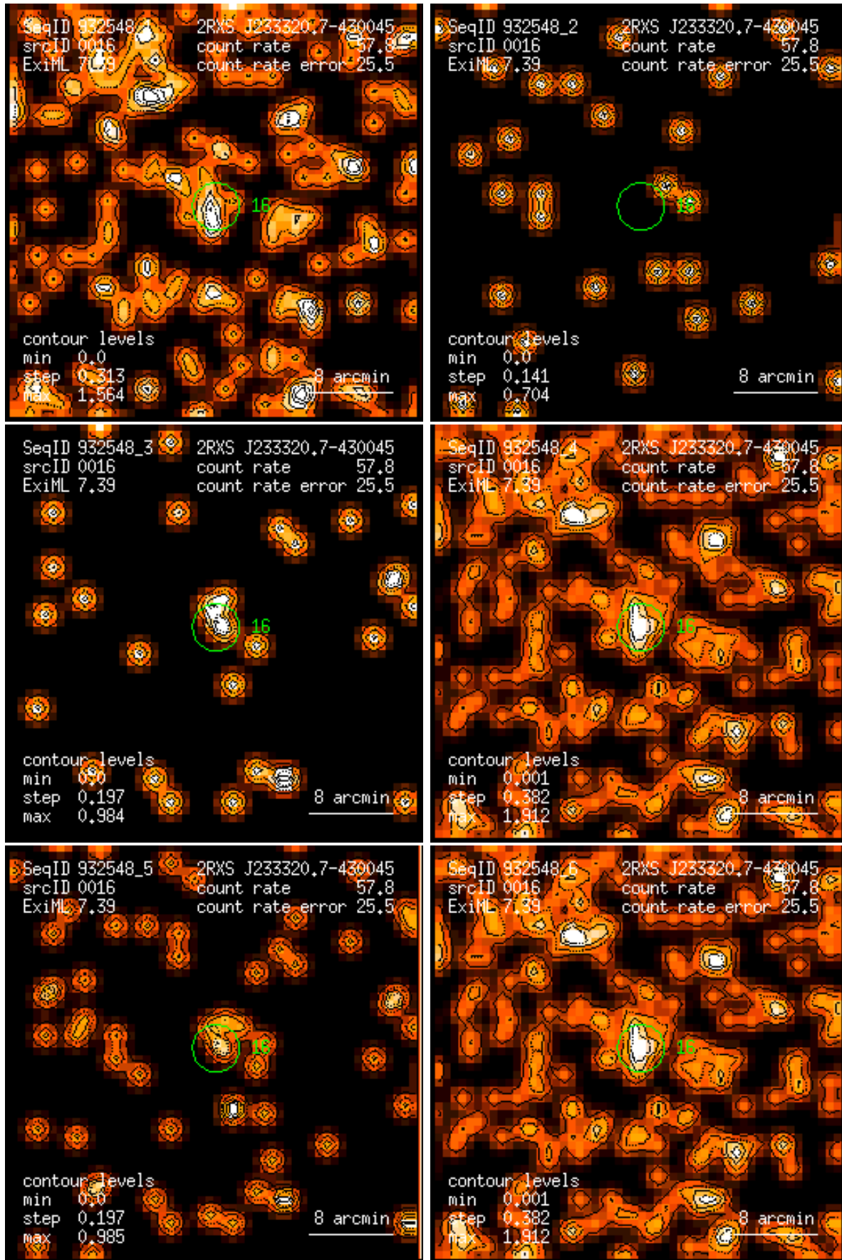
Figure 16: RASS 932548: detection 0016: band rate images, Gaussian filter: (1) PSPC channels 11 – 41, (2) 52 – 90, (3) 91 – 201, (4) 11 – 235, (5) 52 – 201, (6) 11 – 201. Broad band rates in counts/ks. Band rate contour levels in counts/ks/arcmin 2 .
