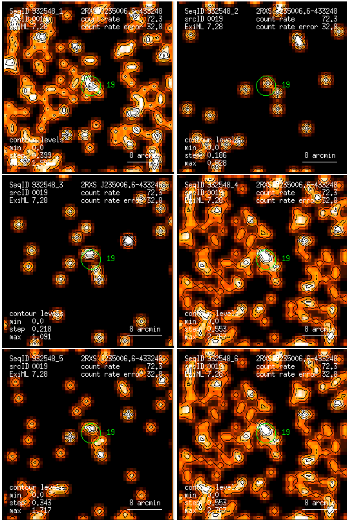
Figure 19: RASS 932548: detection 0019: band rate images, Gaussian filter: (1) PSPC channels 11 – 41, (2) 52 – 90, (3) 91 – 201, (4) 11 – 235, (5) 52 – 201, (6) 11 – 201. Broad band rates in counts/ks. Band rate contour levels in counts/ks/arcmin 2 .
