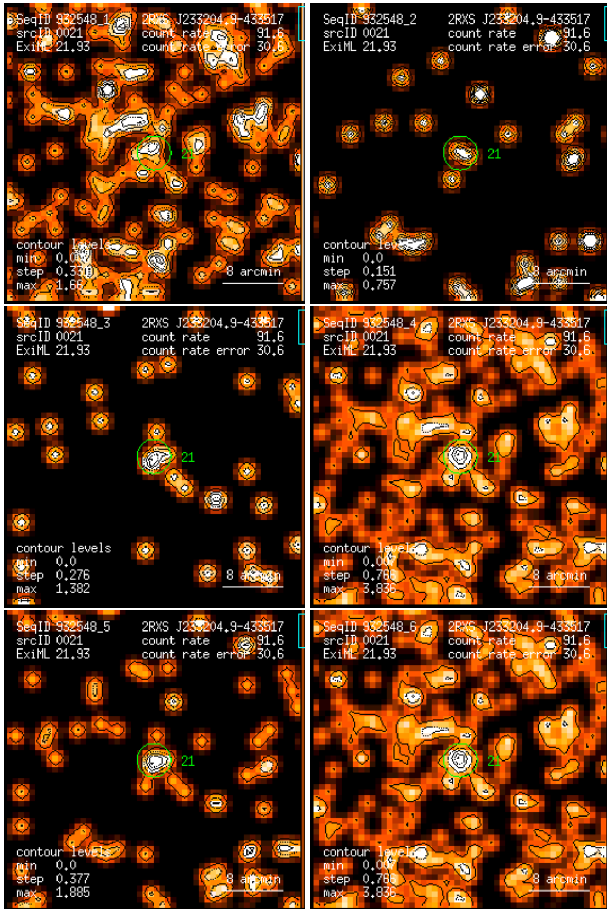
Figure 21: RASS 932548: detection 0021: band rate images, Gaussian filter: (1) PSPC channels 11 – 41, (2) 52 – 90, (3) 91 – 201, (4) 11 – 235, (5) 52 – 201, (6) 11 – 201. Broad band rates in counts/ks. Band rate contour levels in counts/ks/arcmin 2 .
