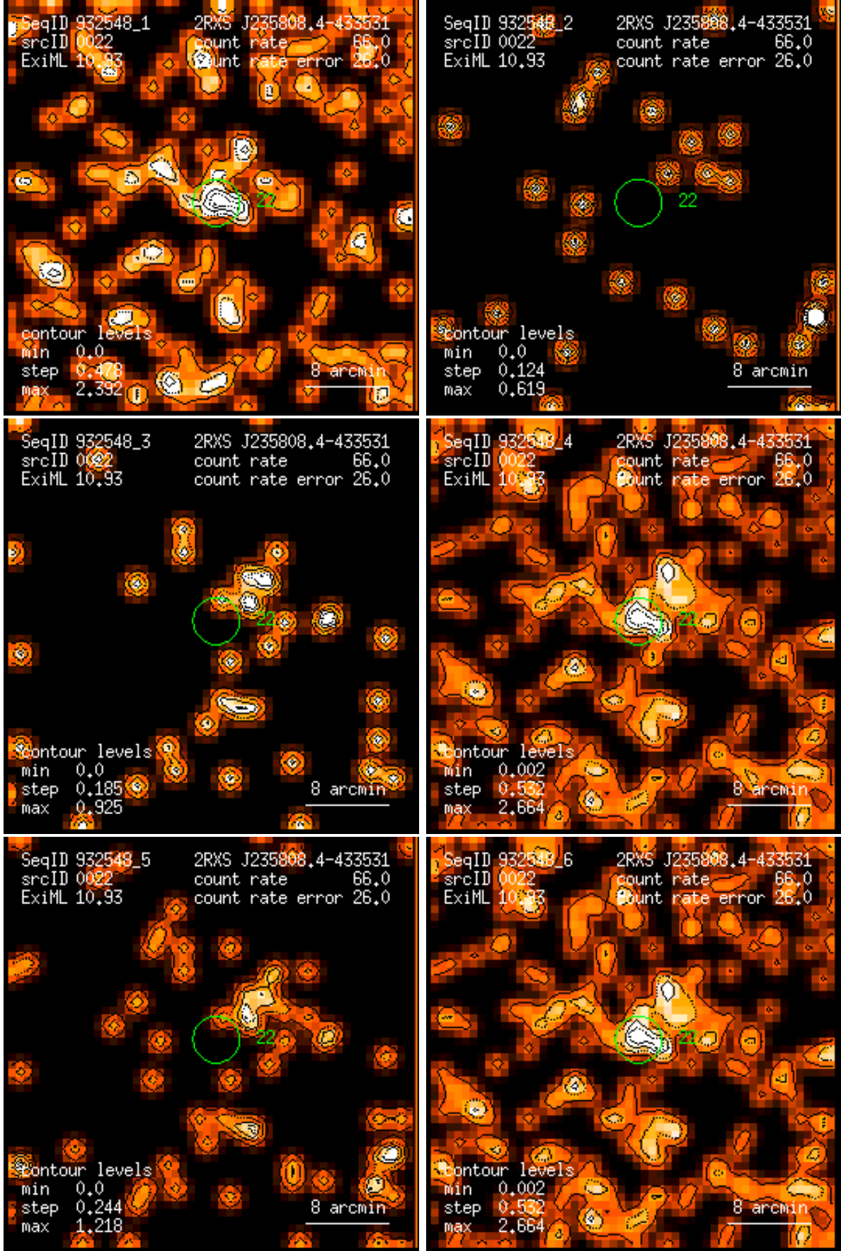
Figure 22: RASS 932548: detection 0022: band rate images, Gaussian filter: (1) PSPC channels 11 – 41, (2) 52 – 90, (3) 91 – 201, (4) 11 – 235, (5) 52 – 201, (6) 11 – 201. Broad band rates in counts/ks. Band rate contour levels in counts/ks/arcmin 2 .
