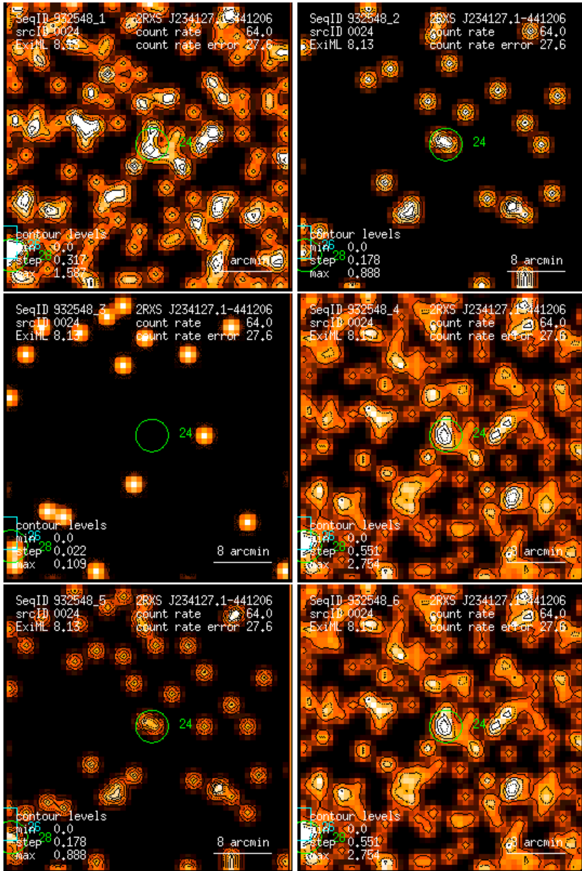
Figure 24: RASS 932548: detection 0024: band rate images, Gaussian filter: (1) PSPC channels 11 – 41, (2) 52 – 90, (3) 91 – 201, (4) 11 – 235, (5) 52 – 201, (6) 11 – 201. Broad band rates in counts/ks. Band rate contour levels in counts/ks/arcmin 2 .
