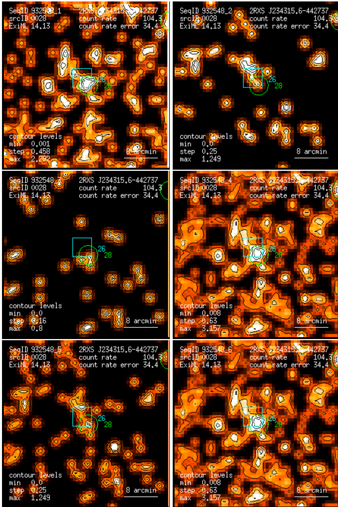
Figure 28: RASS 932548: detection 0028: band rate images, Gaussian filter: (1) PSPC channels 11 – 41, (2) 52 – 90, (3) 91 – 201, (4) 11 – 235, (5) 52 – 201, (6) 11 – 201. Broad band rates in counts/ks. Band rate contour levels in counts/ks/arcmin 2 .
