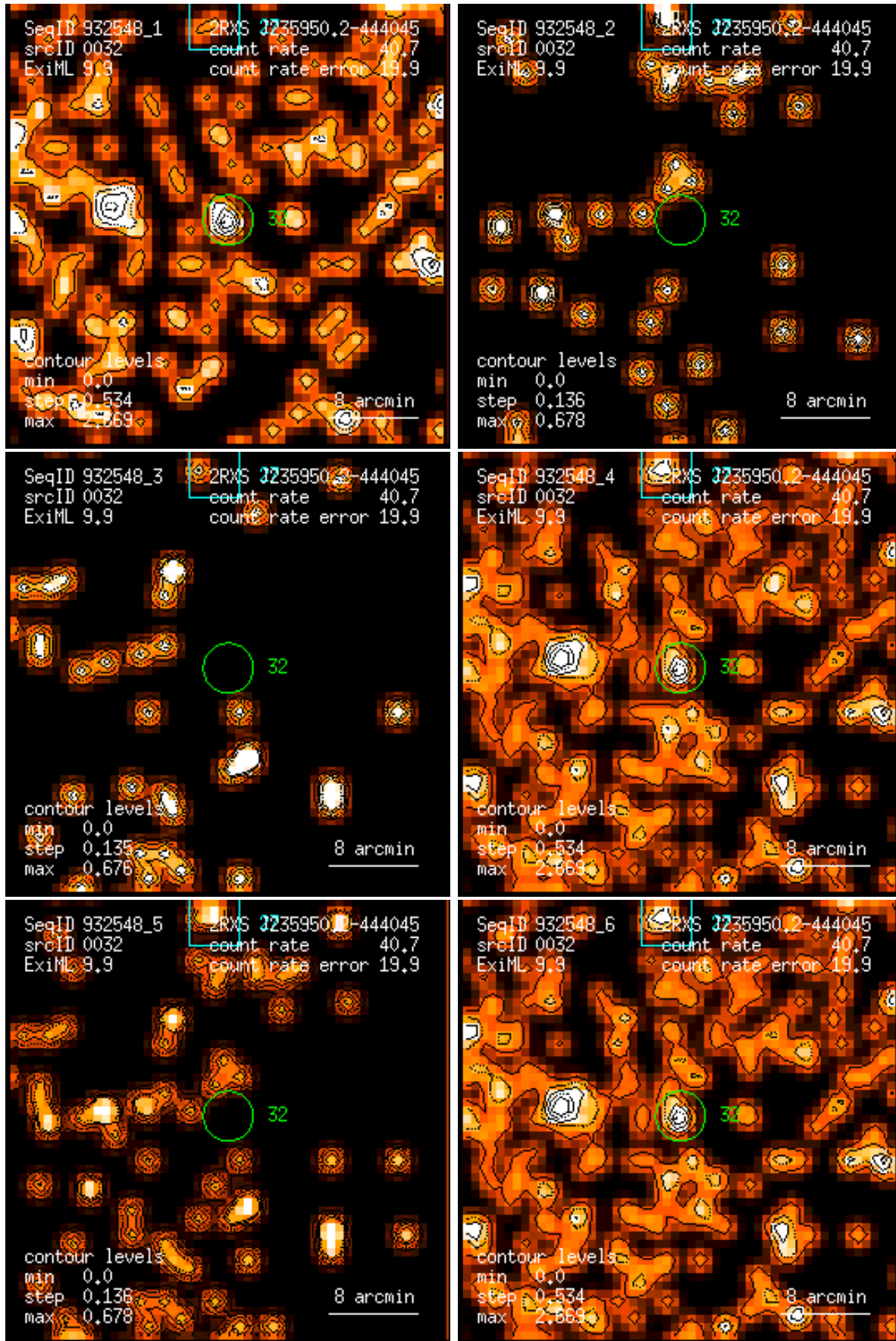
Figure 32: RASS 932548: detection 0032: band rate images, Gaussian filter: (1) PSPC channels 11 – 41, (2) 52 – 90, (3) 91 – 201, (4) 11 – 235, (5) 52 – 201, (6) 11 – 201. Broad band rates in counts/ks. Band rate contour levels in counts/ks/arcmin 2 .
