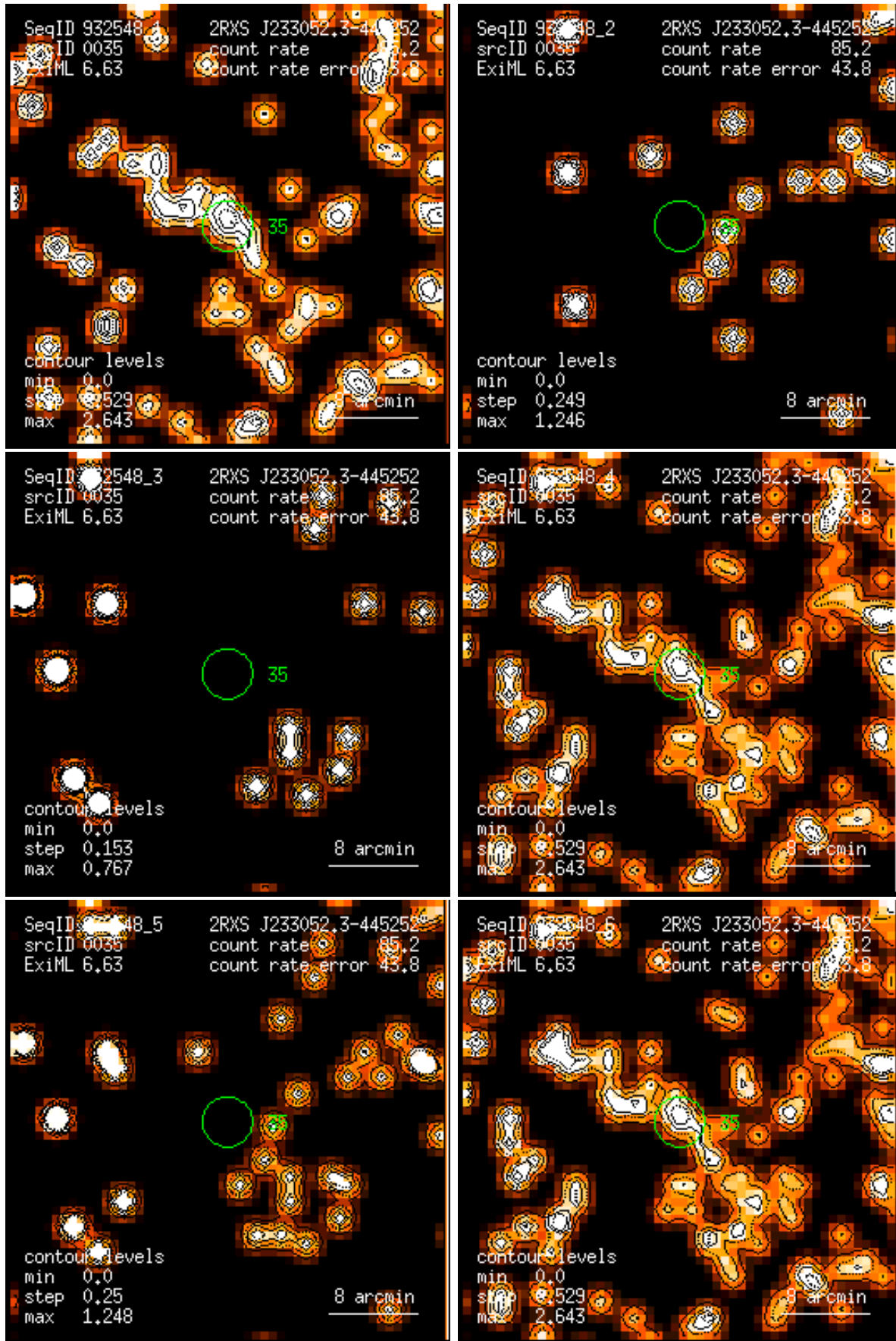
Figure 35: RASS 932548: detection 0035: band rate images, Gaussian filter: (1) PSPC channels 11 – 41, (2) 52 – 90, (3) 91 – 201, (4) 11 – 235, (5) 52 – 201, (6) 11 – 201. Broad band rates in counts/ks. Band rate contour levels in counts/ks/arcmin 2 .
